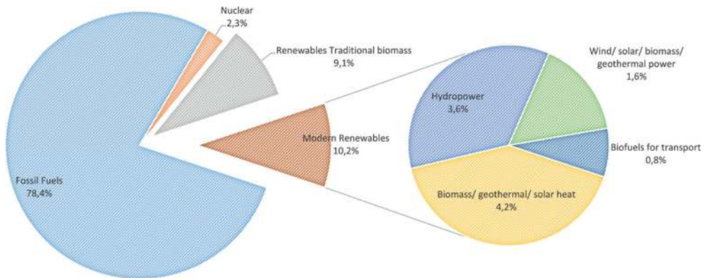
Figure 5. Global renewable energy share (data from [33]).
