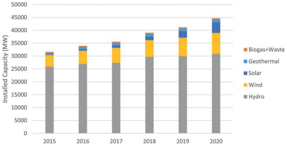
Figure 8. Installed renewable capacity projection in Turkey (data collected from [42] and interpreted).
