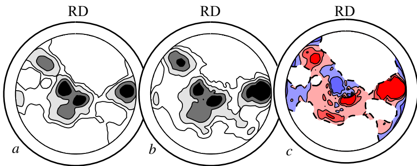
Figure 11. Recrystallization in cold rolled \alpha -Zr single crystals N 3 ( \epsilon \sim 30\% (a-c) and \epsilon \sim 70\% (d-f)): a - PF(0001)_{roll} ; b - PF(0001)_{recr} ; c - [PF(0001)_{recr} - PF(0001)_{roll}] .
