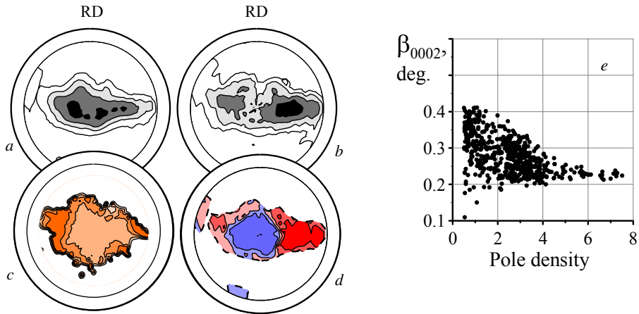
Figure 14. Recrystallization of polycrystalline rolled iodide \alpha -Zr ( \epsilon -50%): a - PF(0001) roll ; b - PF(0001) recr ; c - GPF \beta_{0002} ; d - [PF(0001) recr - PF(0001) roll ]; e - diagram of correlation PF(0001) - GPF \beta_{0002} .
