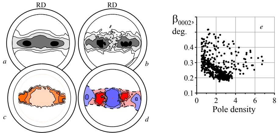
Figure 16. Recrystallization of Zr-1%Nb alloy rolled along initial RD ( \epsilon -50%): a - \text{PF}(0001)_{\text{roll}} ; b - \text{PF}(0001)_{\text{recr}} ; c - \text{GPF } \beta_{0002} ; d - [\text{PF}(0001)_{\text{recr}} - \text{PF}(0001)_{\text{roll}}] ; e - diagram of correlation \text{PF}(0001) - \text{GPF } \beta_{0002}
