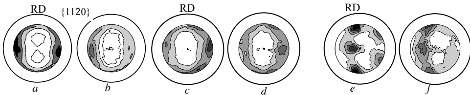
Figure 13. Texture changes through the recrystallization of rolled \alpha -Zr single crystals N 1, \epsilon =80% (a, b), N 2, \epsilon =70% (c, d) and N 3, \epsilon = 70% (e, f). (a, c, e): PF {11 \bar{2} 0} for rolled single crystals; (b, d, f):PF {11 \bar{2} 0} for rolled and annealed single crystals 580°C/3 h.
