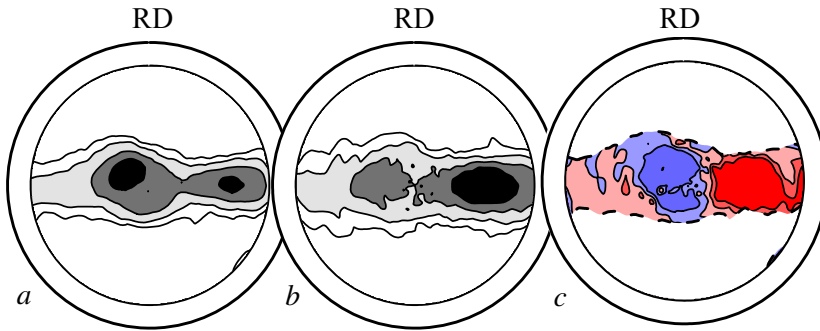
Figure 12. Recrystallization in cold rolled \alpha -Zr single crystals N 3 ( \epsilon -30% (a-c) and \epsilon -70% (d-f)): a- PF(0001) roll , b - PF(0001) recr ; c - [PF(0001) recr - PF(0001) roll ].
