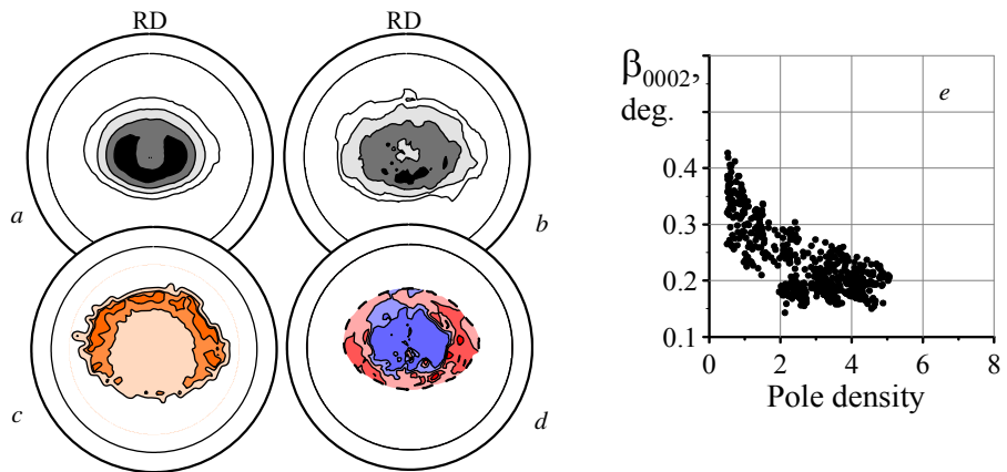
Figure 17. Recrystallization of Zr-1%Nb alloy rolled across initial RD ( \epsilon -50%): a - \text{PF}(0001)_{\text{roll}} ; b - \text{PF}(0001)_{\text{recr}} ; c - \text{GPF } \beta_{0002} ; d - [\text{PF}(0001)_{\text{recr}} - \text{PF}(0001)_{\text{roll}}] ; e - diagram of correlation \text{PF}(0001) - \text{GPF } \beta_{0002}
