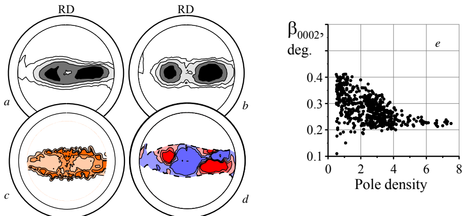
Figure 15. Recrystallization of polycrystalline rolled iodide \alpha -Zr ( \epsilon -80%): a - PF(0001) roll ; b - PF(0001) recr ; c - GPF \beta_{0002} ; d - [PF(0001) recr - PF(0001) roll ]; e - diagram of correlation PF(0001) - GPF \beta_{0002} .
