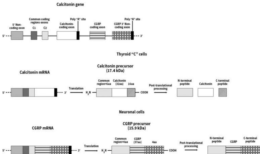
Figure 2. Calcitonin or CGRP production from CALC I gene.
