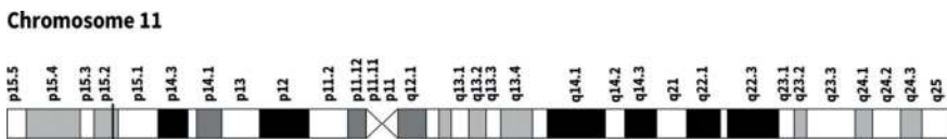
Figure 3. The structure of CALCA gene.
