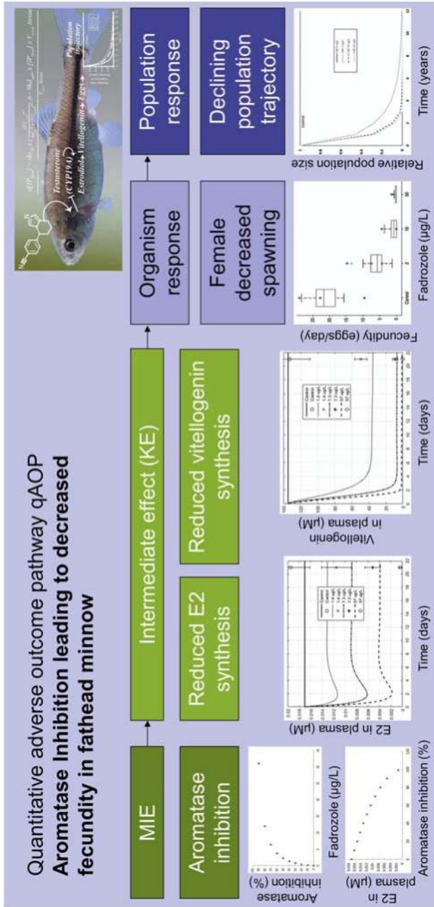
Figure 9.10 Development of a quantitative adverse outcome pathway (qAOP) in fathead minnow on the example of the anti-breast cancer drug fadrozole. MIE = molecular initiating event; E2 = 17 \beta -estradiol; KE = key event. Reprinted after modification with permission from Conolly et al. (2017). Quantitative adverse outcome pathways and their application to predictive toxicology. Environmental Science & Technology , 51 (8): 4661–4672. © 2017. American Chemical Society.
