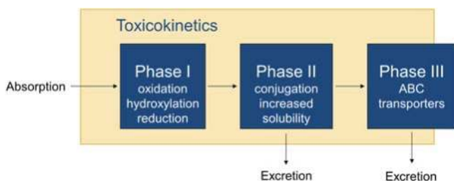
Figure 4.2 Three phases of xenobiotic metabolism in a cell in relation to the other toxicokinetic processes of absorption and excretion.
