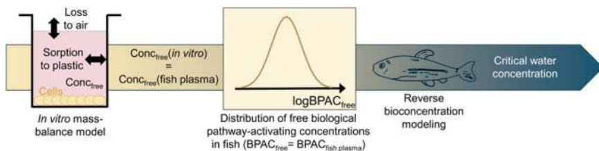
Figure 9.9 Extrapolating in vitro concentration–response to equivalent in vivo effect in fish analogously to the QIVIVE model for Judson et al. (2011) presented in Figure 9.4. Plasma concentrations in fish estimated based on the free fraction of the active chemical concentration in the assay test well. Reverse bioconcentration modelling can then be used to estimate the water concentration that would yield the equivalent internal dose. Modified and reprinted with permission from Villeneuve et al. (2019). High throughput screening and environmental risk assessment – state of the science and emerging applications. Environmental Toxicology and Chemistry , 38 (1): 12–26. © 2019. John Wiley and Sons.
