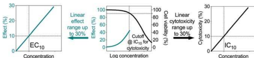
Figure 7.9 Derivation of inhibitory concentration causing 10% cytotoxicity IC_{10} and effect concentration causing 10% effect EC_{10} from the linear portion of the CRC. Modified from Escher et al. (2018). Reprinted with permission by John Wiley and Sons © 2018.
