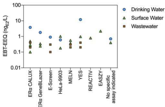
Figure 13.11 Overview of published EBT values for estrogenic activity in units of 17\beta -estradiol equivalent concentration (EEQ, \text{ng}_{\text{E}_2}/\text{L} ) for drinking water (circles), surface water (triangles) and wastewater effluent (squares). See Table 13.1 for numerical values and more details.
