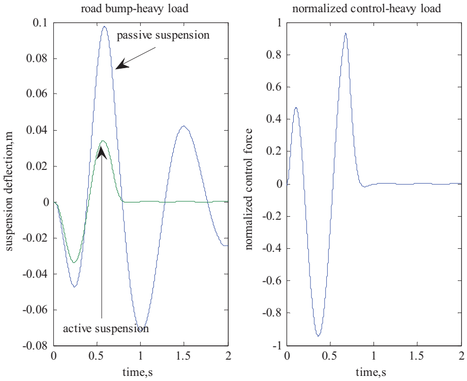
Figure 9. Road bump response at heavy load.
