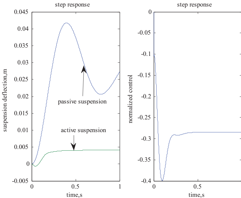
Figure 6. Step response at light load.
