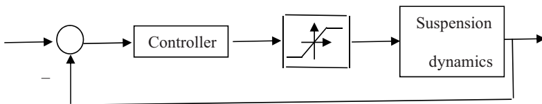
Figure 2. Feedback-saturated control systems.
