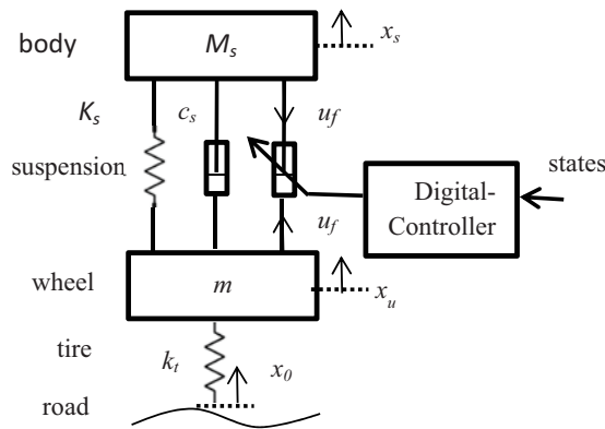
Figure 1. Quarter-car model with an active suspension.
