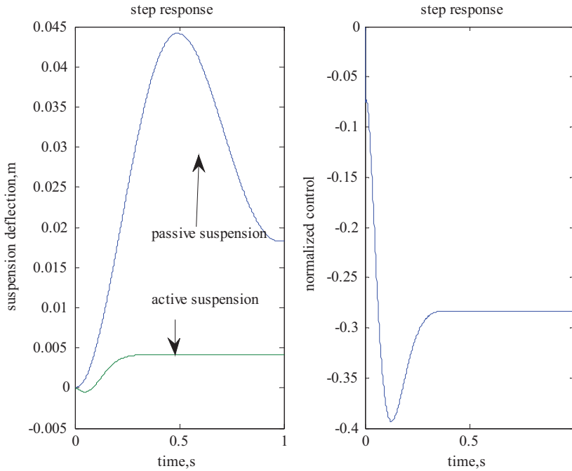
Figure 7. Step response at heavy load.
