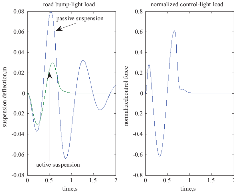
Figure 8. Road bump response at light load.
