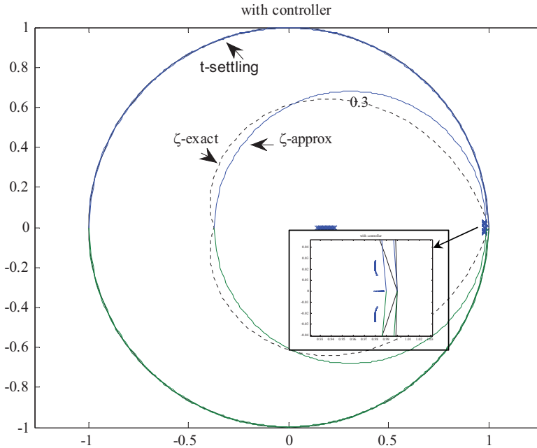
Figure 5. Closed-loop poles with system uncertainties using saturated control.
