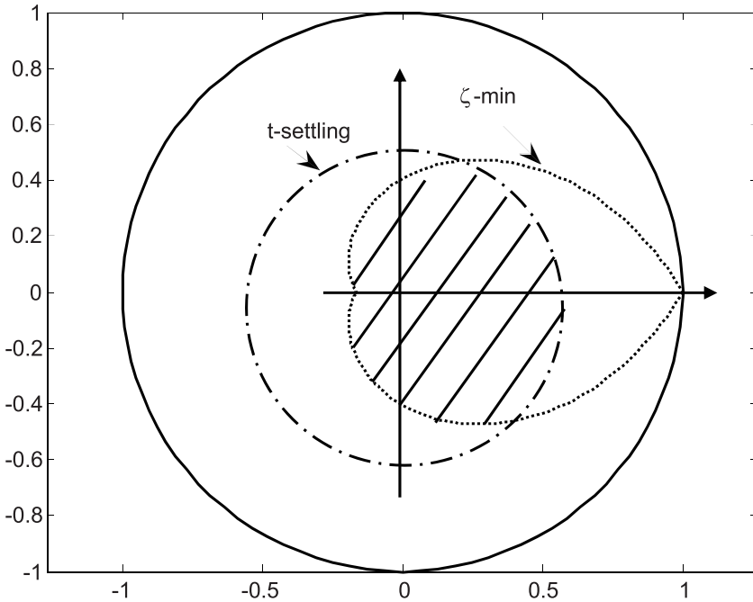
Figure 3. Desired region of closed-loop poles, hatched.
