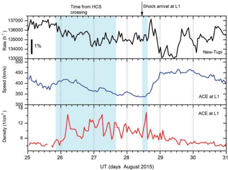
Figure 10. Comparison between the muon counting rate in the New-Tupi telescope (top panel) and the solar wind parameters (density and speed) observed by the ACE satellite (center and bottom panels) in the period from August 25 until August 31. The shaded area indicates the HCS crossing time and the vertical arrow show the arrival of a shock associated with a high-speed stream on August 28.
