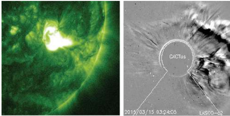
Figure 2. Left panel: Register of the long duration C9.1 peaking at 02:13 UT (March 15, 2015) around sunspot 2297. Credit: SDO/AIA. Right panel: Register of the partial CME associated to the C9.1 arc. Credit: C2 Lasco.
