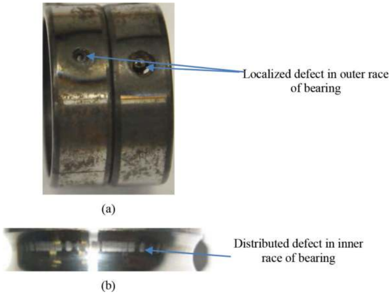
Figure 6. Example of bearing (a) localized defects and (b) distributed defects.
