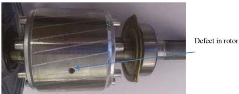
Figure 10. Example of rotor fault in induction motor [13].
