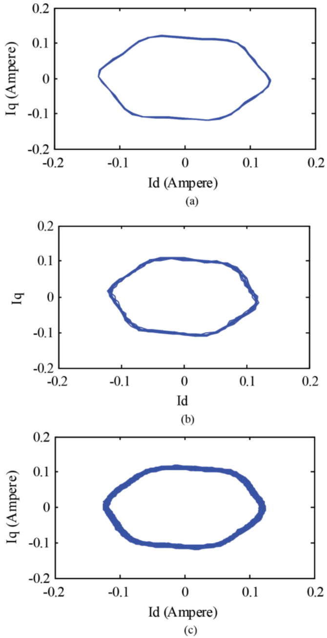
Figure 14. Example of Park vector analysis of stator current for (a) healthy bearing, (b) outer race localized defect and (c) inner race localized defect.
