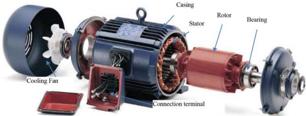
Figure 3. The structure of induction motor [5].
