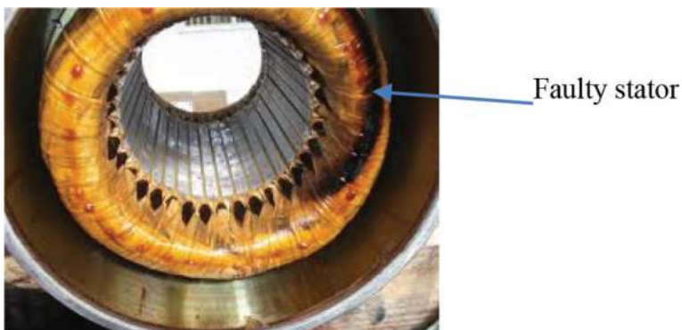
Figure 9. The stator fault in induction motor [31].
