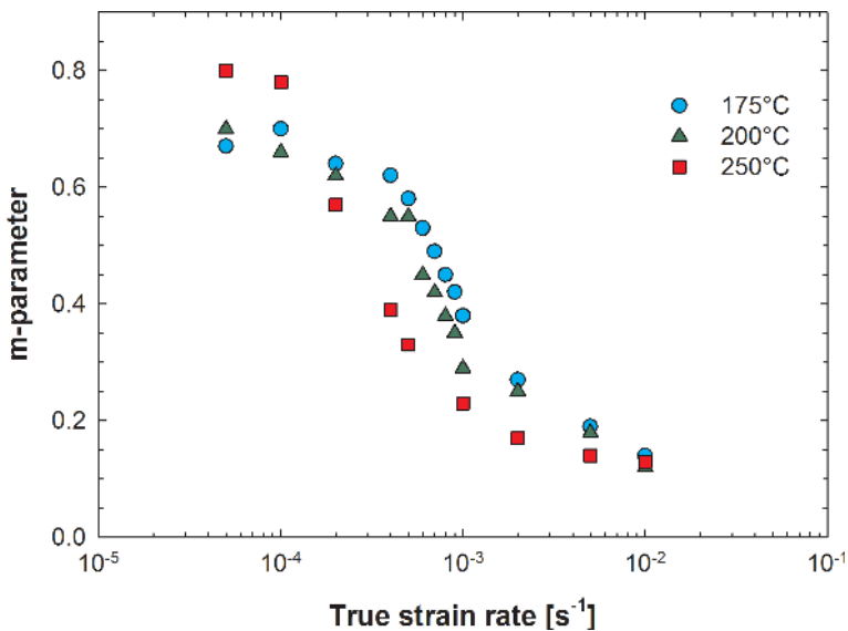
Figure 9. Measured m -parameter at deformation temperatures 175, 200, and 250°C.
