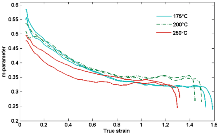
Figure 11. Evolution of m -parameter determined from interpolated flow curves for samples deformed at 175, 200, and 250°C.
