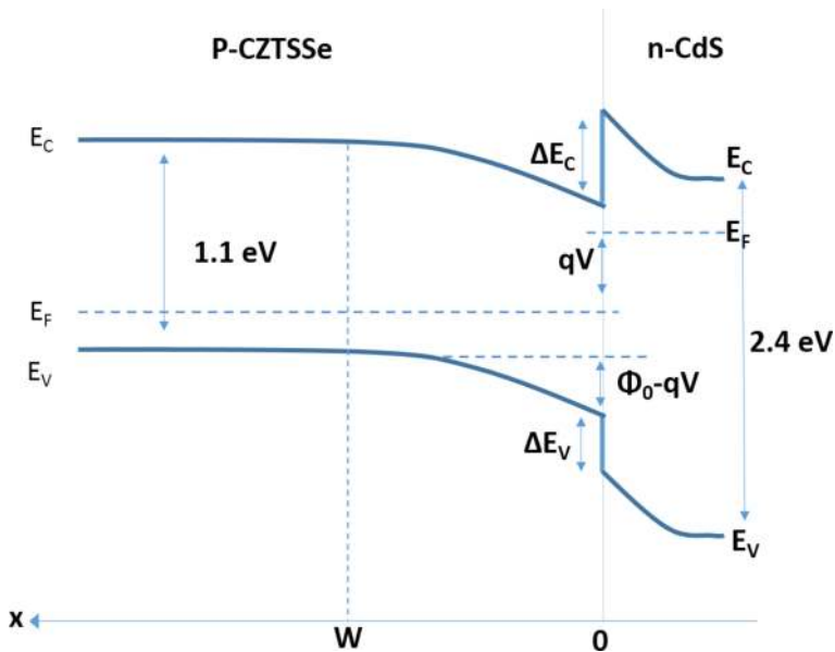
Figure 2. Energy band diagram of n-CdS/p-CZTSSe heterojunction at biased condition (V).
