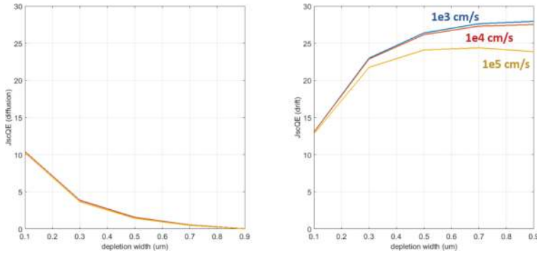
Figure 6. JscQE (drift) and JscQE (diffusion) under the standard AM 1.5 solar radiation (1 sun, 100 mW/cm 2 ) under different front surface recombination velocities (10 3 , 10 4 , and 10 5 cm/s).
