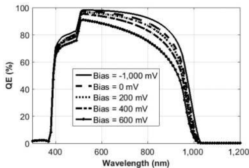
Figure 8. Q-E of ideal CZTSSe solar cells without interface defects at bias conditions ( -1.0 , 0.0 , 0.2 , 0.4 , and 0.6 V ).
