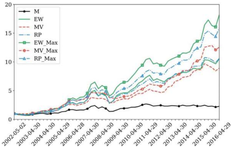
Figure 5. Cumulative return curves for KOSPI 200 data.
