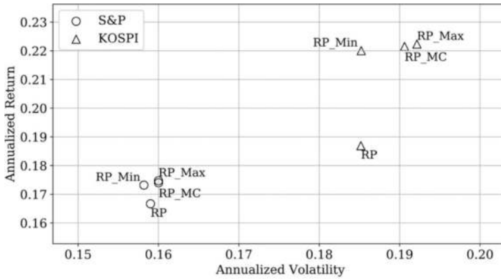
Figure 3. Annualized return versus volatility for RP-based strategies.
