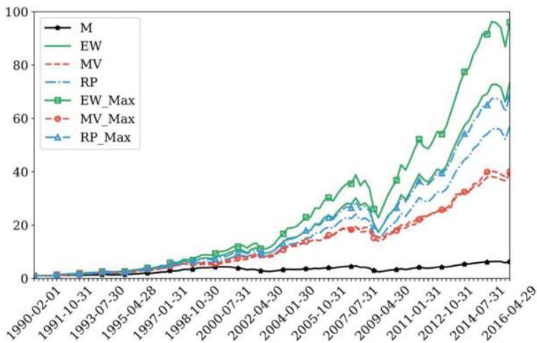
Figure 4. Cumulative return curves for S&P 500 data.
