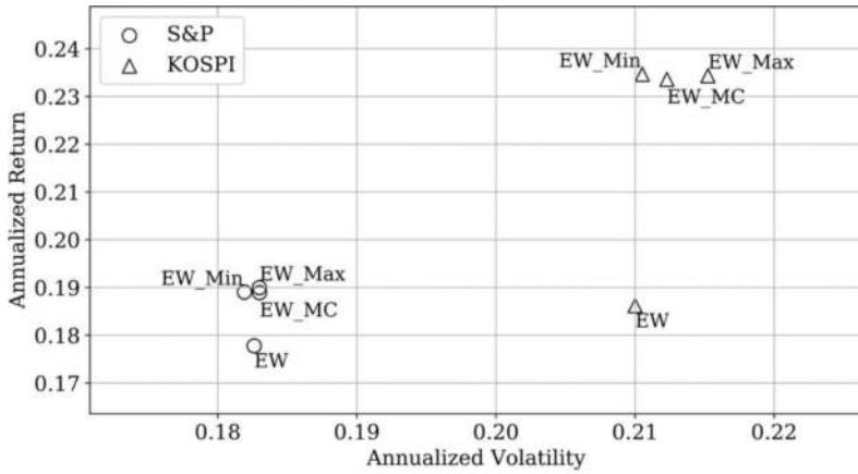
Figure 1. Annualized return versus volatility for EW-based strategies.
