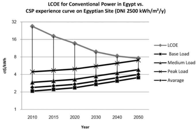
Figure 14. Egypt LCOE (CSP) vs. conventional power.
