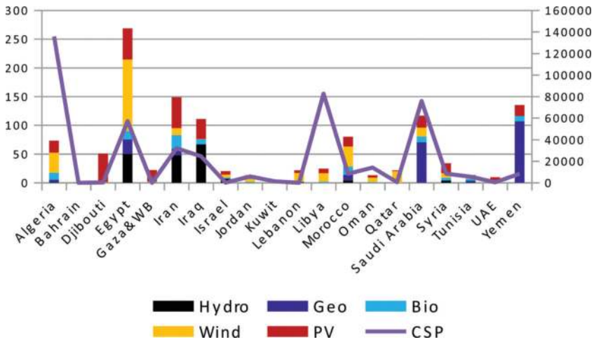
Figure 7. Renewable power generation potential by sources in TWh/y [15].
