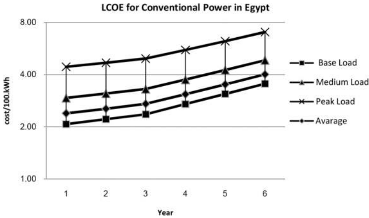
Figure 13. LCOE for conventional power in Egypt.
