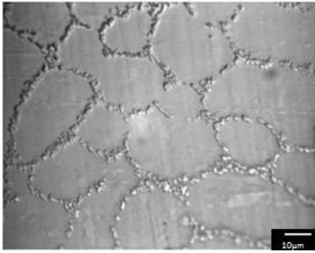
a. SAC305 as reflow condition
