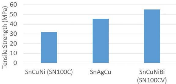
Figure 8. Tensile strength comparison for three alloys in as-cast condition.
