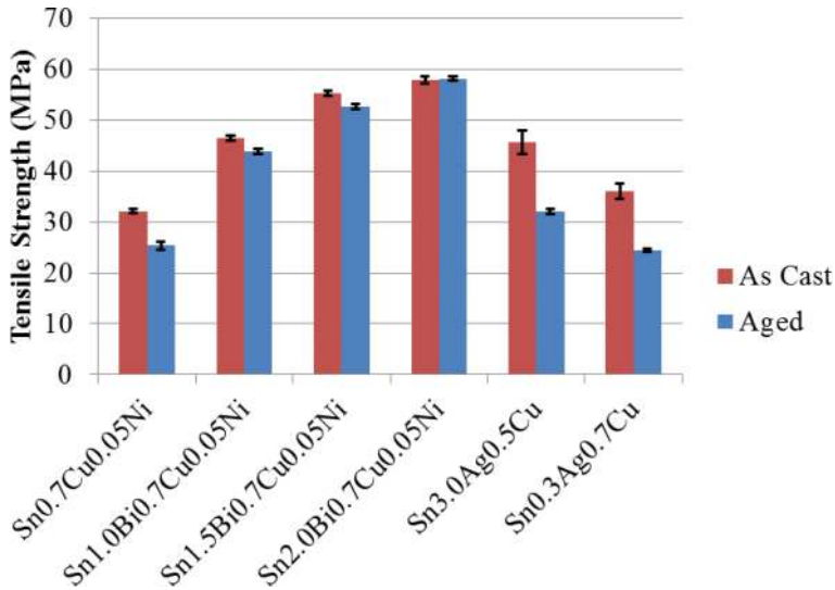
Figure 10. Tensile strength of test alloys as-cast and after thermal aging at 150°C for 500 h.
