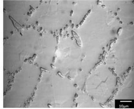
b. SAC305 after 6 months exposure to 125°C isothermal aging
