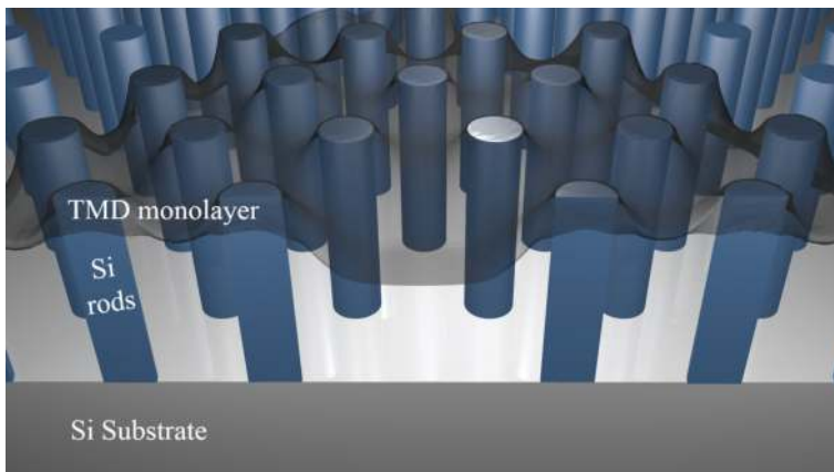
Figure 1. Cross-sectional illustration of a silicon rod PhC cavity with a monolayer transferred on top. Declining of the monolayer within the cavity region can increase coupling between excitons and the cavity modes.
