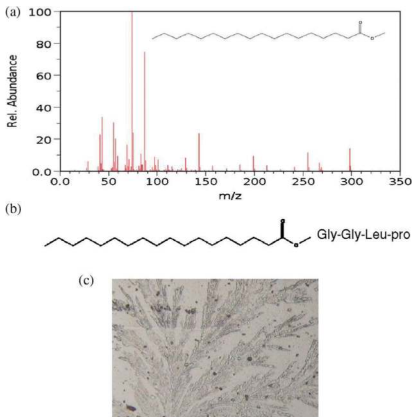
Figure 1. MS spectra of octadecanoic acid methyl ester (a), probable structure of octadecanoic acid methyl ester with peptide moiety (b), crystalline appearance of the recovered crystals of lipopeptide (MSA13) examined under a light microscope at 40x [23].
