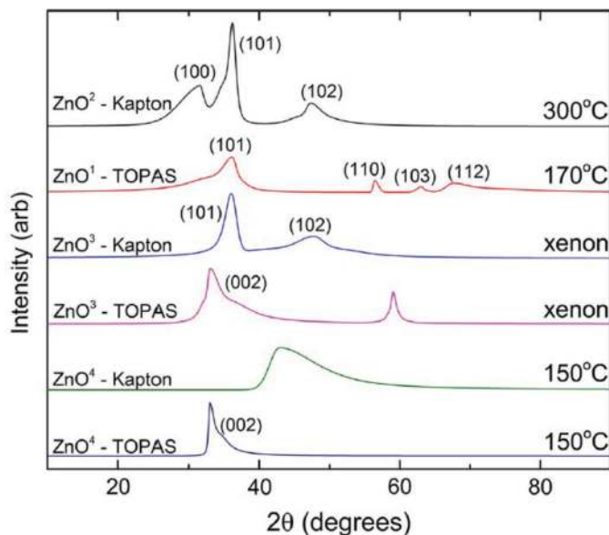
Figure 6. XRD spectra for IJP films on Kapton and TOPAS substrates sintered by hot plate and xenon arc lamp [20].
