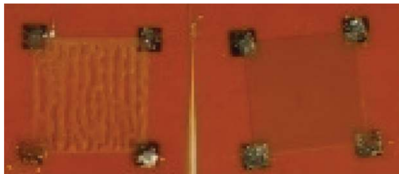
Figure 10. Comparison of ZnO thin films printed by IJP ( left, ZnO 2 ) and AJP ( right, ZnO 7 ) sintered at 300°C. The printed silver pads and indium contacts were applied to the corners for Hall effect measurements. Image taken by a Samsung Galaxy S6 [20].
