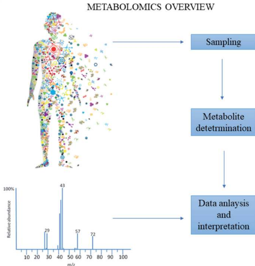
Figure 1. Metabolomic workflow.
