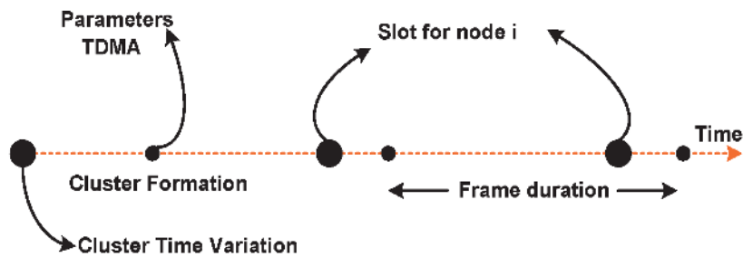
Figure 8. Operation of APTEEN.
