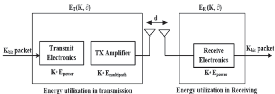
Figure 4. Energy radio model.
