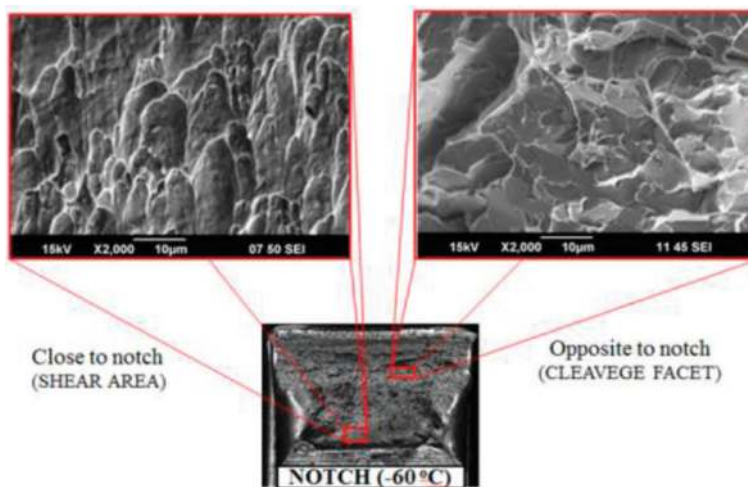
Figure 18. Fracture surface for 10-mm thick CVN specimen tested at -60^{\circ}\text{C} .
