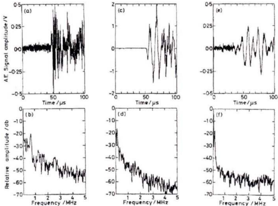
Figure 3. Waveforms and corresponding frequency spectra [13].
