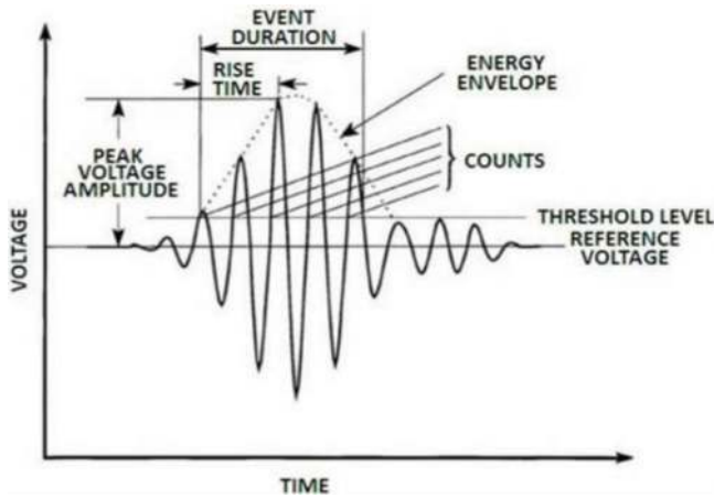
Figure 2. Parameters of an AE hit [6].
