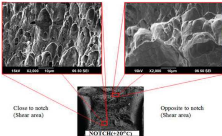
Figure 17. Fracture surface for 10-mm thick CVN specimen tested at +20°C.
