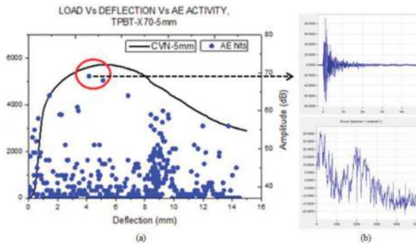
Figure 20. (a) AE activity corresponding to the load-deflection curve obtained during TPBT; (b) selected AE signal waveform and power spectrum corresponding to the fracture initiation for 5-mm thick CVN sample.
