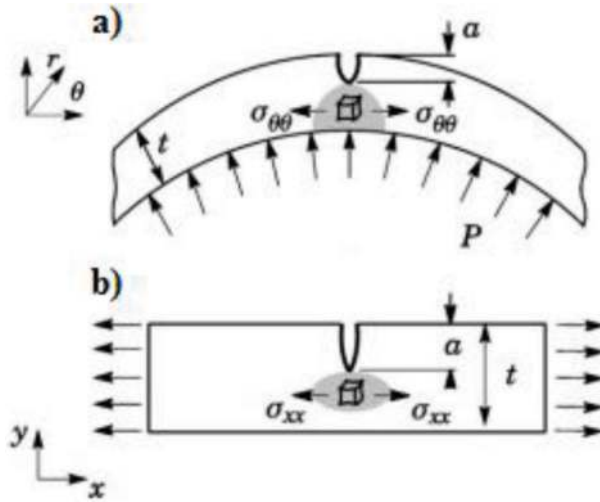
Figure 11. (a) Schematic loading condition for a pressurized pipe; (b) SENT test specimen [38].
