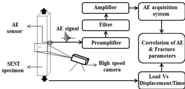
Figure 9. A schematic of AE measurement setup of SENT testing.
