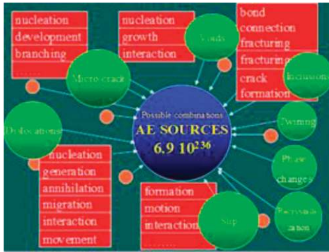
Figure 4. AE sources in steel micro and macrostructure [10].
