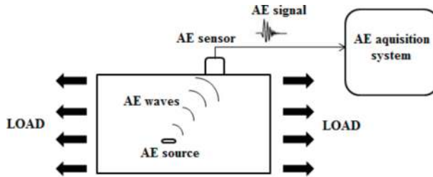
Figure 1. Schematic presentation of AE monitoring technique.
