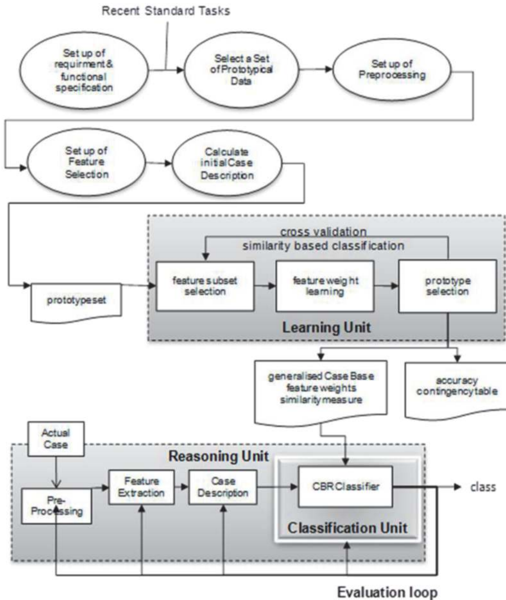
Figure 1. Methodology.
