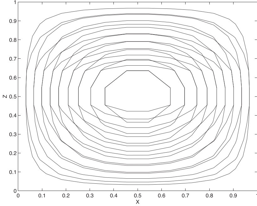
Figure 3. Illustration of the contact zone.
