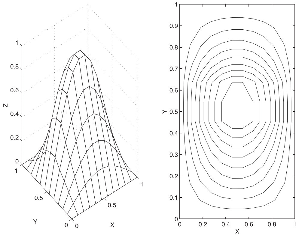
Figure 2. Approximate solution u_h^{(0)} .
