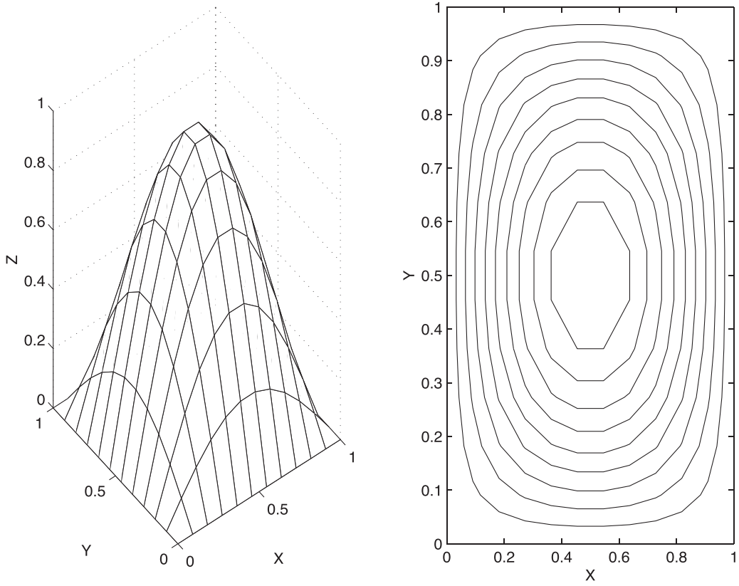
Figure 1. Obstacle function \psi .
