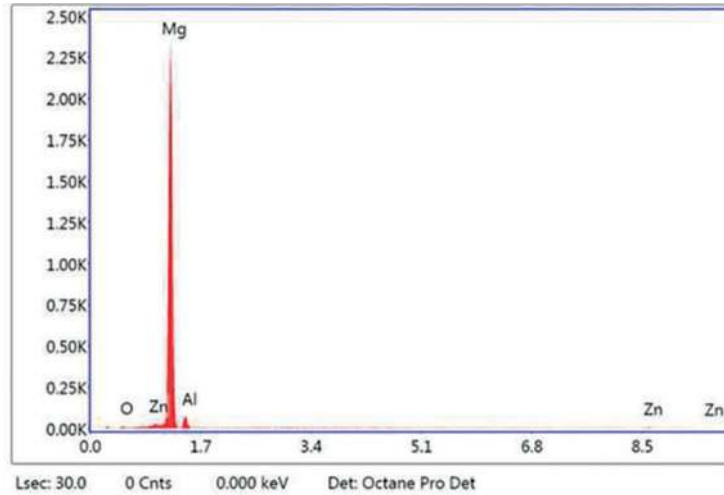
Figure 2. EDS spectrum of AZ91/1% Al 2 O 3 nanocomposites.
