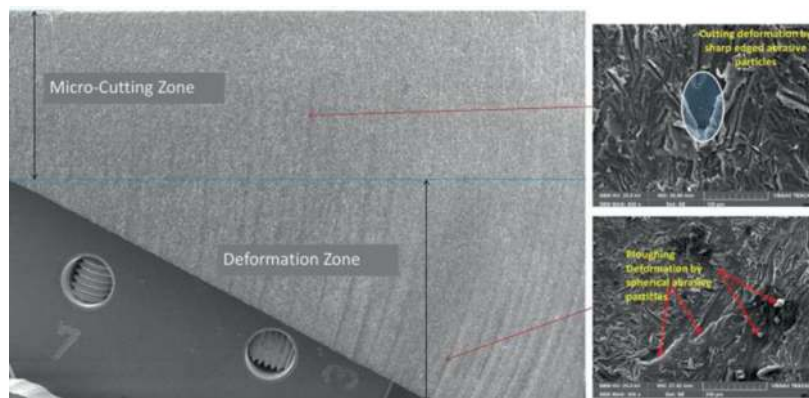
Figure 4. Material removal mechanism.
