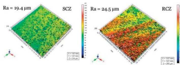
Figure 6. 3-D images of SCZ and RCZ.
