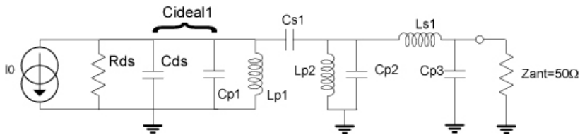
Fig. 10. Equivalent circuit of the driver and transistor.
