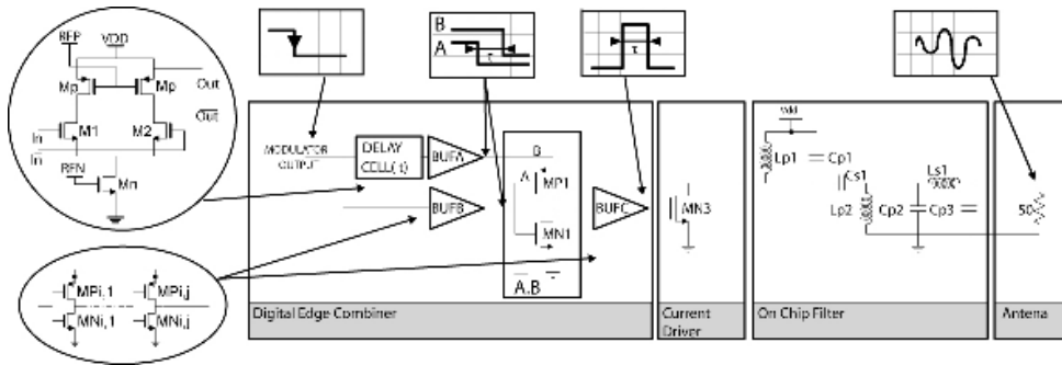
Fig. 9. Architecture of the FCC generator.
