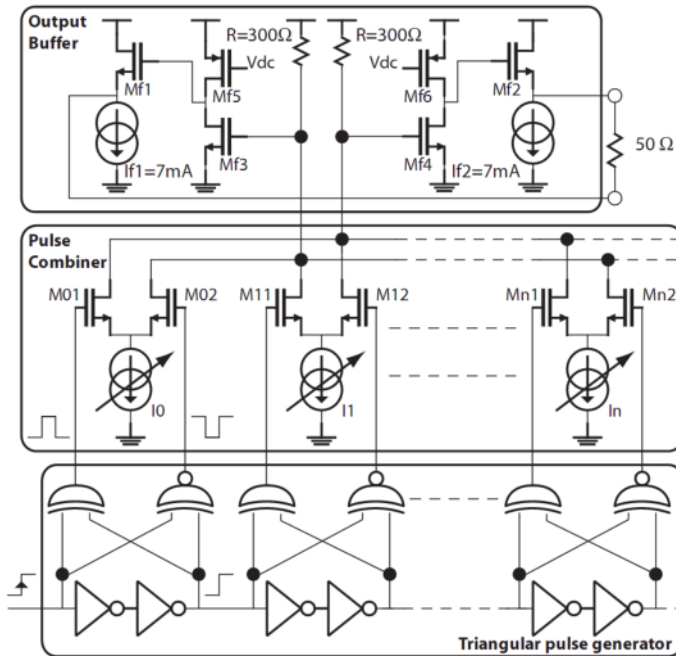
Fig. 12. Principle of combination using cross-connected differential pairs.
