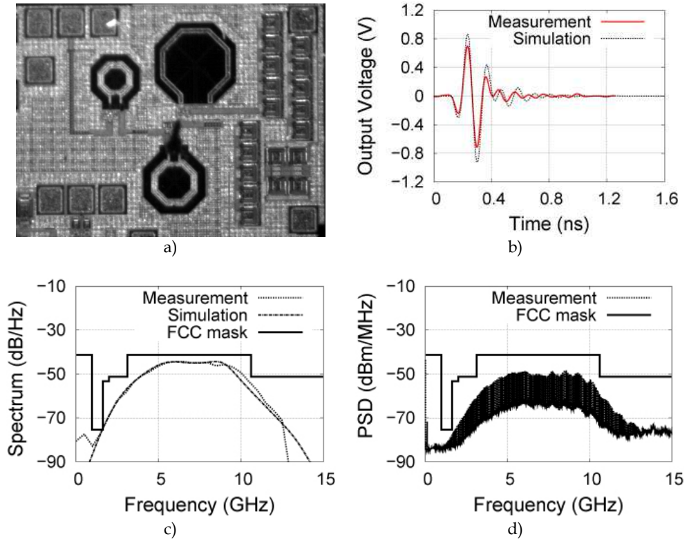
Fig. 11. Measurement results for the FCC generator.
