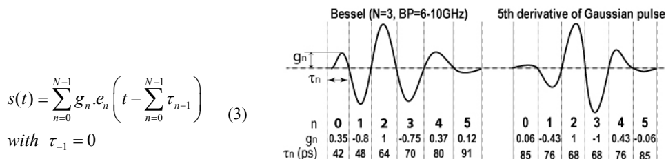
Fig. 3. Principle of synthesis by pulse combination.
