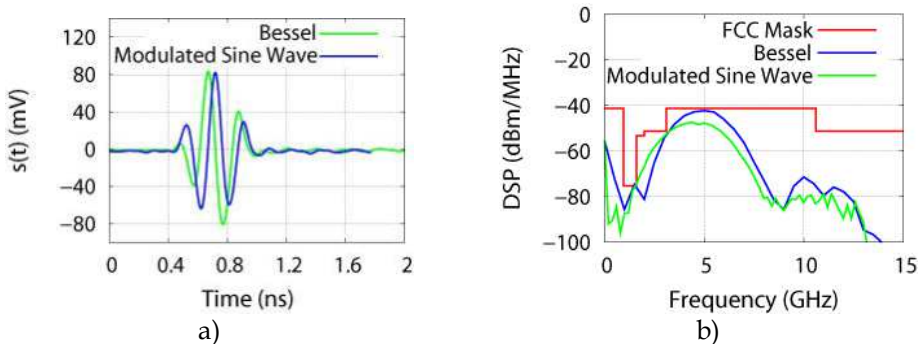
Fig. 15. Measurement of the various elementary pulses a) and their spectrum b).
