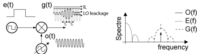
Fig. 1. Principle of frequency transposition architectures
