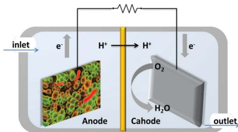
Figure 2. Scheme of working principle of microbial fuel cells (MFCs).
