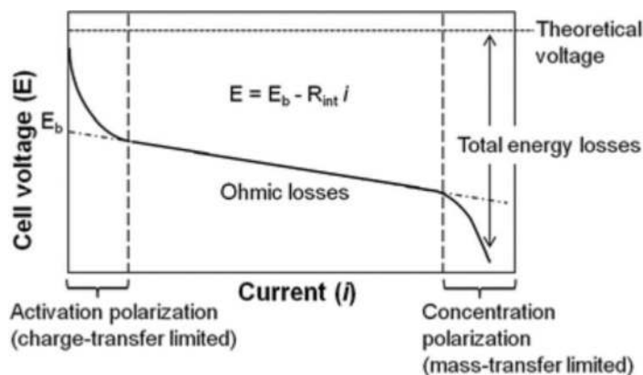
Figure 4. The polarization curve for typical MFCs. Reprinted with the permission from (chemical society reviews, 2012, 41, 7228–7246) copyright (2012) Royal Society of Chemistry.
