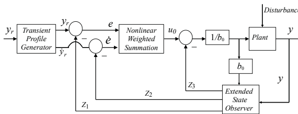
Fig. 1. The control block based on the ADRC
