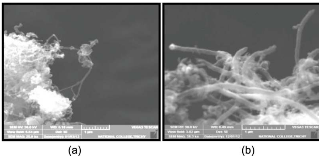
Figure 7. (a and b) SEM images of MWNTS grown at the flow rate of 10 and 30 mL.
