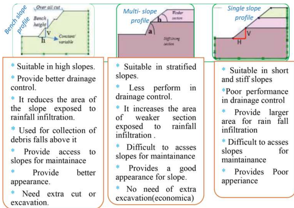
Figure 11. Advantages and limitations of slope profiles.
