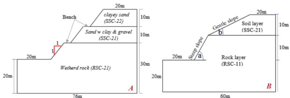
Figure 3. Cross-section of the newly constructed road cut slope.
