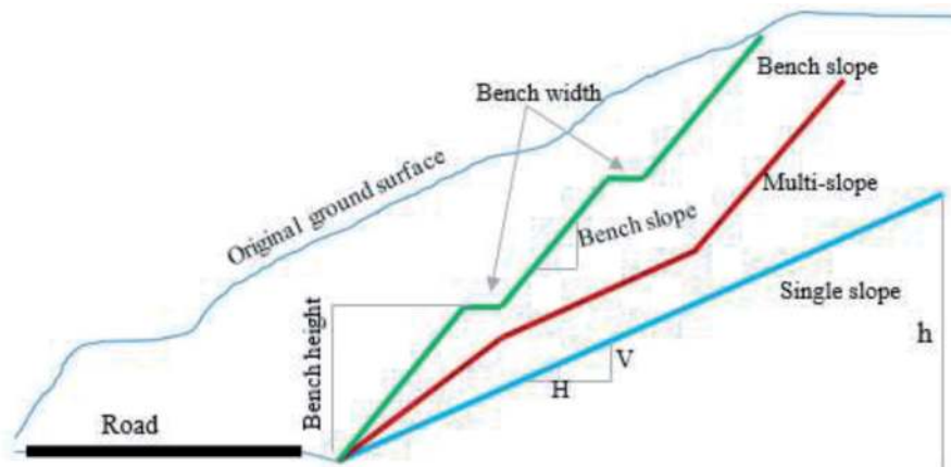
Figure 2. Geometric profiles of cut slope.
