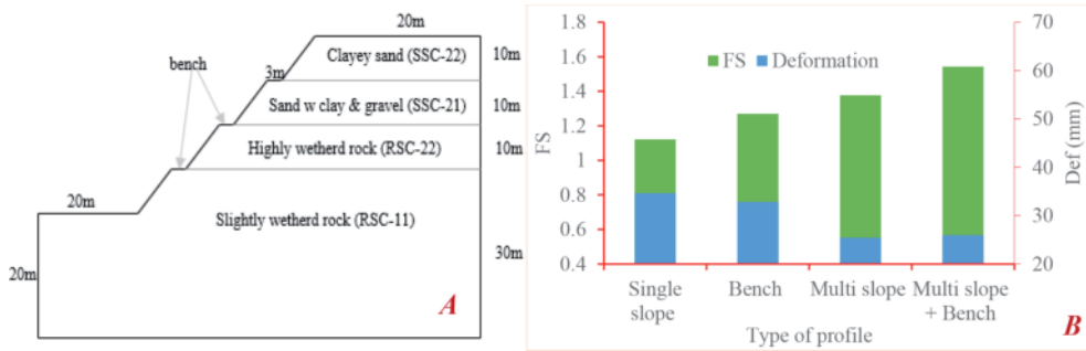
Figure 10. FS and deformation for different slope profiles.
