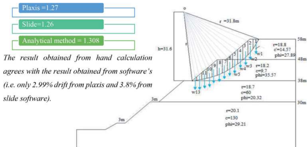
Figure 4. FS determination using analytical solutions.
