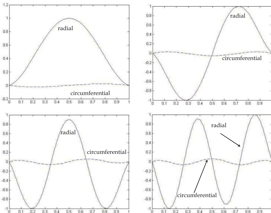
Fig. 4. First four ormalized modes for clamped-clamped curved symmetric sandwich beam
