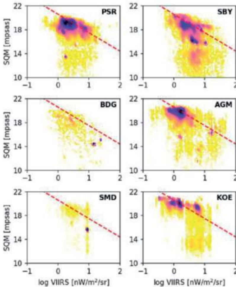
Figure 12. Density plot of SQM data obtained during the trip by each team correlated with map from VIIRS which put in logarithmic scale. Dashed line represents empirical model from [14].
