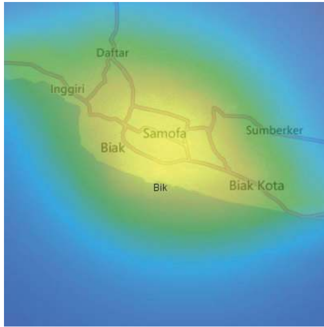
Figure 10. Light pollution at Biak station.
