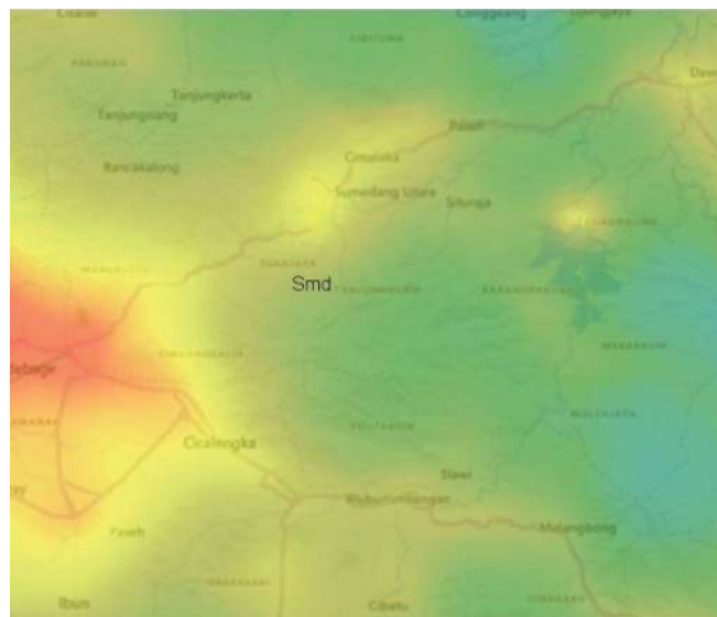
Figure 7. Light pollution at Sumedang station.
