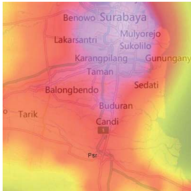
Figure 9. Light pollution at Pasuruan station.
