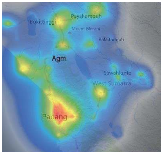
Figure 4. Light pollution at Agam station.
