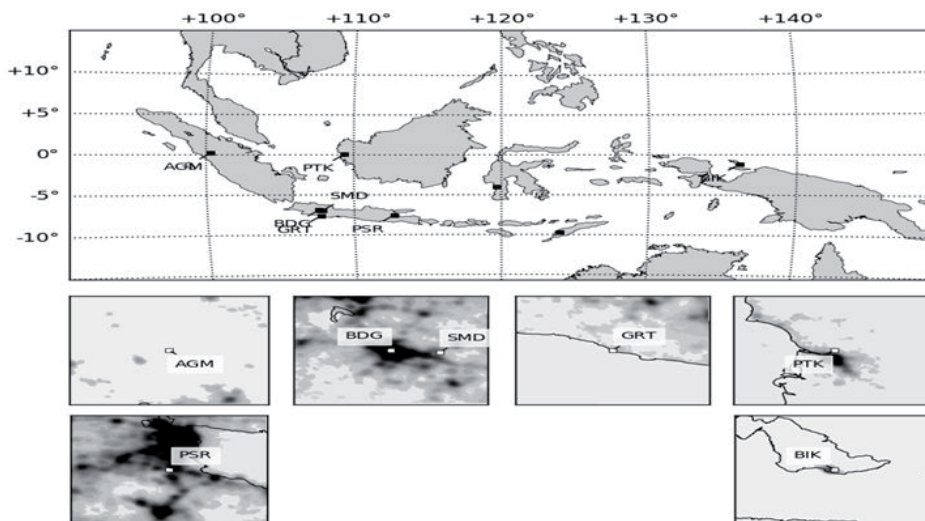
Figure 1. Locations of sky quality observations in Indonesia.
