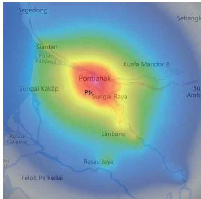
Figure 5. Light pollution at Pontianak station.
