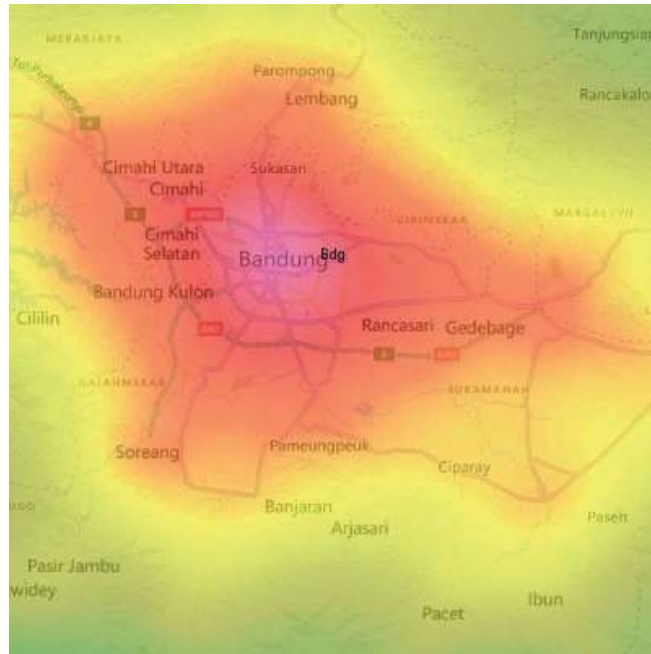
Figure 6. Light pollution at Bandung station.
