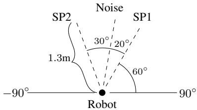
Fig. 9. Illustration of setup of expts. 3 and 4.
