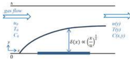
Figure 2. Schematic illustration of a classical boundary layer and reactor conditions over the susceptor.
