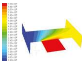
Figure 1. Temperature distribution profile simulated by commercial FLUENT ® software for an ASM Epsilon One CVD reactor when the total pressure is ATM. The hydrogen gas is considered to be the main gas flowing over the susceptor, in order to simplify the simulation. The susceptor is heated up by an assembly of lamps to the deposition temperature (here 700°C) [19].
