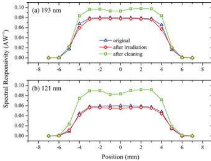
Figure 16. Measured responsivity across the surface in one direction of a 9.6×9.6 mm 2 LT PureB photodiode at wavelengths of 193 and 121 nm, before and after high-dose exposure, and after cleaning. The high-dose exposure was performed with a circular beam spot of \phi 1 mm with a radiant exposure of 37 J/cm 2 [22].
