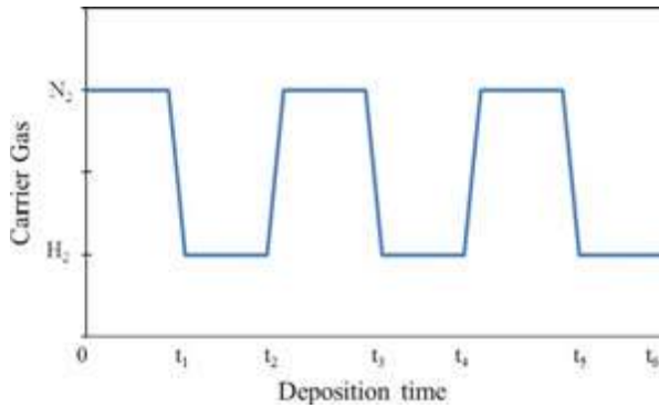
Figure 8. Schematic illustration of carrier gases switching sequences in the LT PureB recipe [22].
