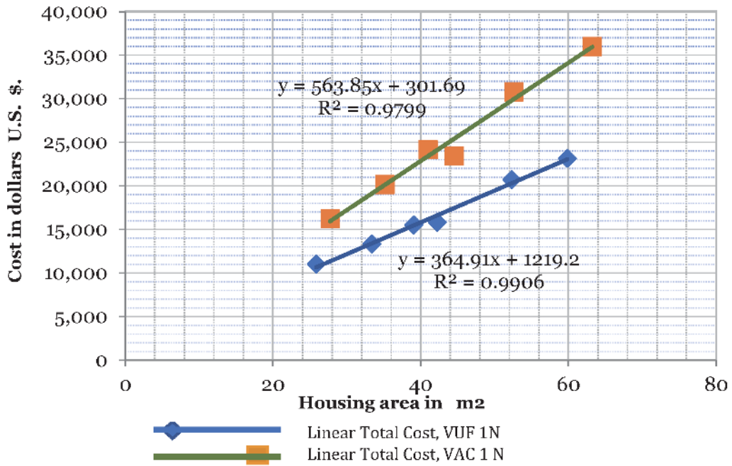
Figure 15. Linear Total cost of VUF and VAC.
