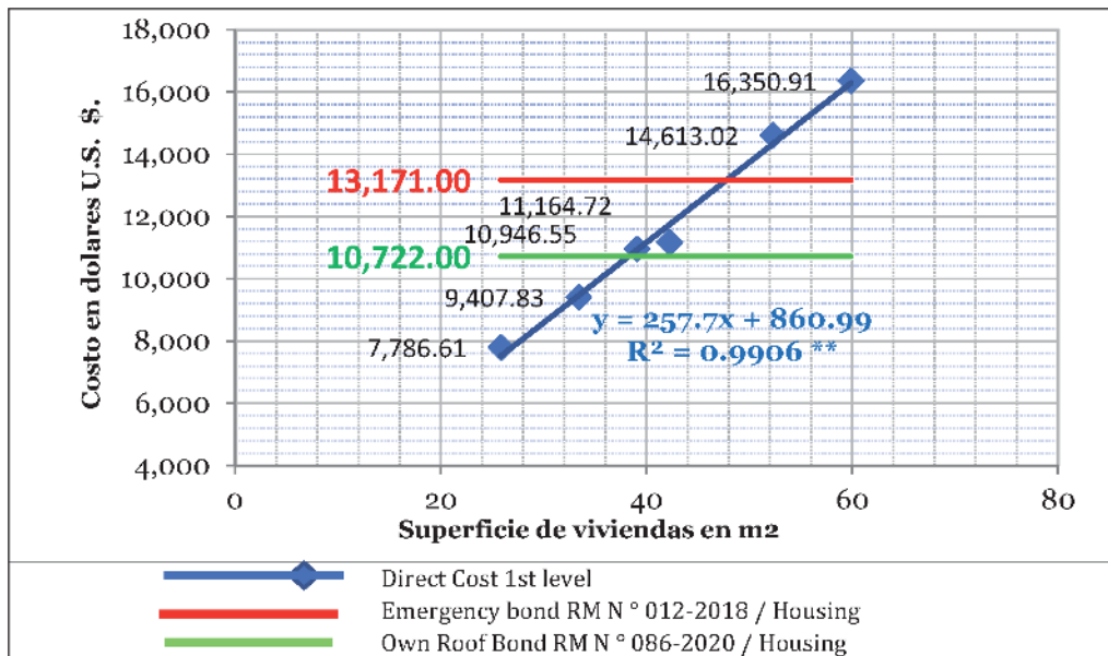
Figure 12. Direct cost of VUF and its relationship to emergency bonds.
