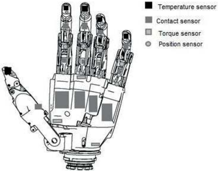
Figure 2. Example of the arrangement of sensors on the hand artificial limb.
