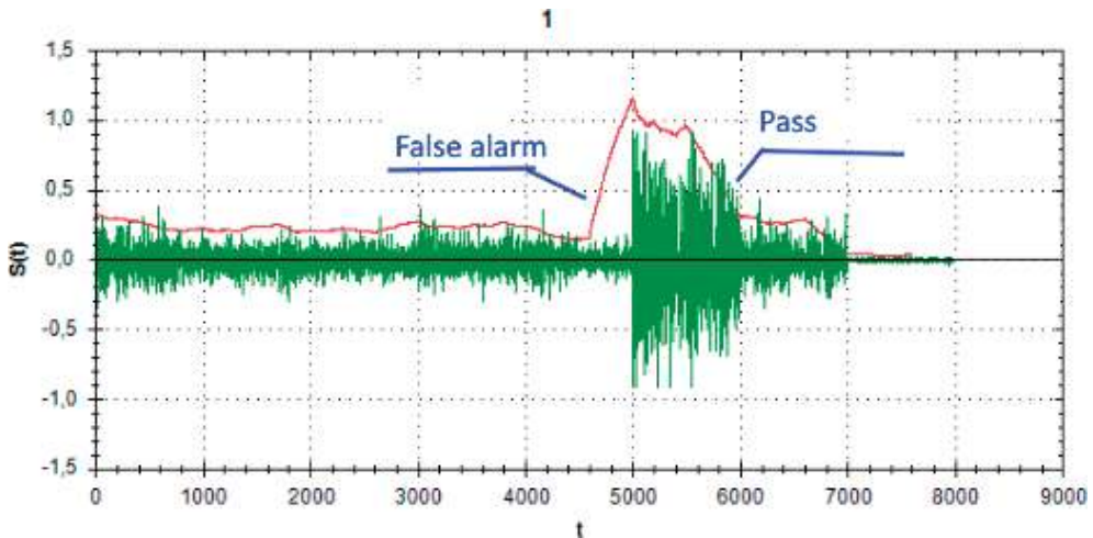
Figure 13. The bending-around signal EMG.
