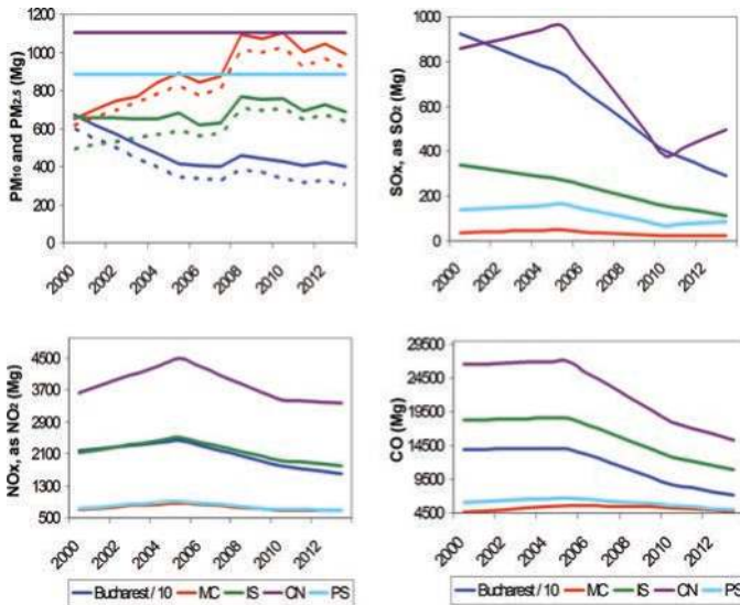
Figure 3. Pollutant emission trends per site as resulted from WebDab emission database, for national total economic sectors. Dotted lines represent PM_{2.5} emissions. Bucharest emissions are included for comparison.
