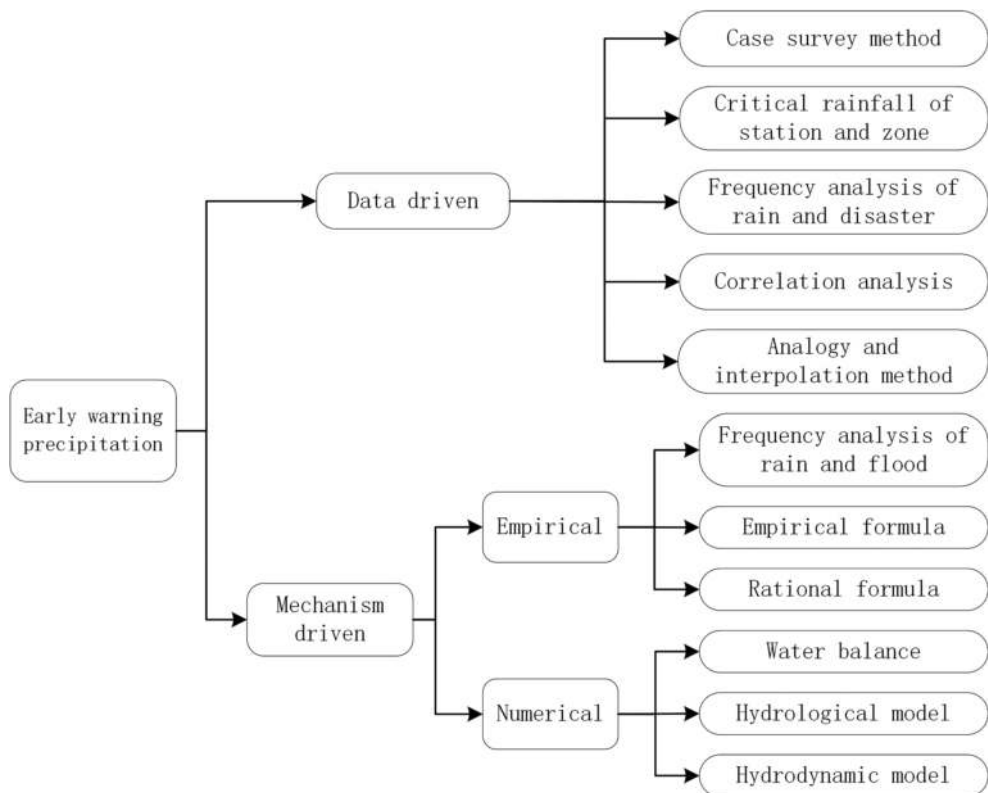
Figure 3. The methods of calculating early warning rainfall.
