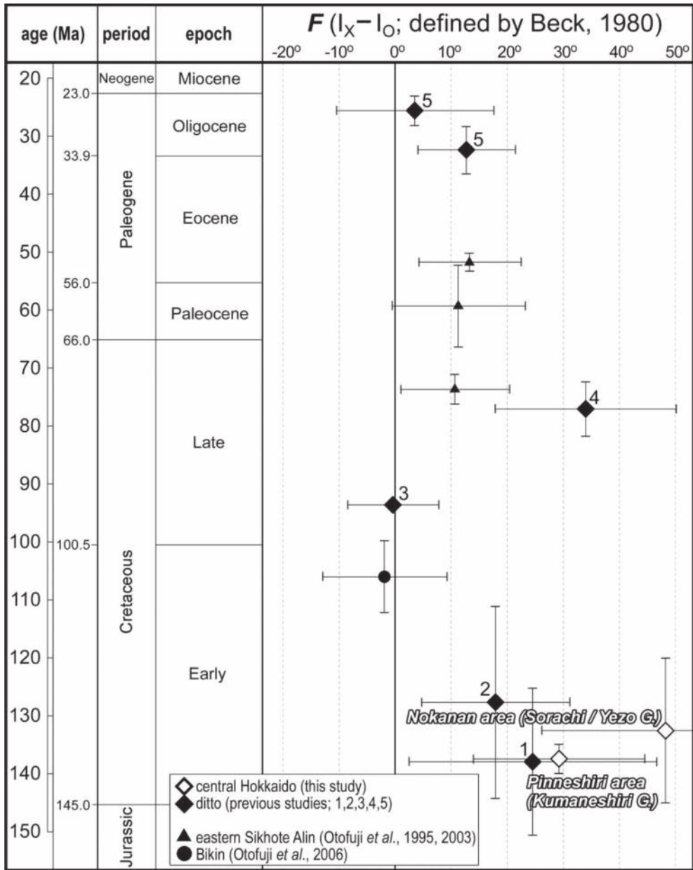
Figure 10. Plot of inclination flattening ( F ) ( F = I [expected] - I [observed]; [24]) versus age for central Hokkaido (1 = [10]; 2 = [11]; 3 = [7]; 4 = [4]; 5 = [33]), eastern Sikhote Alin and Bikin. Stratigraphic positions of data in eastern Sikhote Alin and Bikin are after Otofujii et al. [34, 35] and Otofujii et al. [36], respectively. The age range of the Oyubari data (3: [7]) is shorter than the height of the median symbol.
