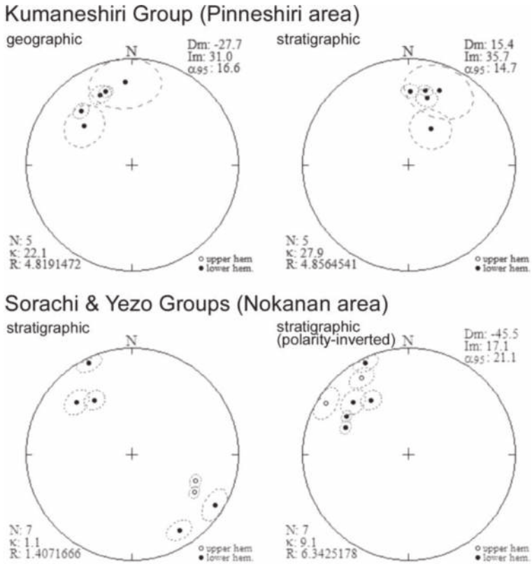
Figure 4. Site-mean directions of high T_{UB} components of the Kumaneshiri, Sorachi, and Yezo Groups in geographic and stratigraphic coordinates on equal-area projections. Solid (open) symbols are on the lower (upper) hemisphere of the equal-area projections. Dotted ovals are 95% confidence limits of site-means.
