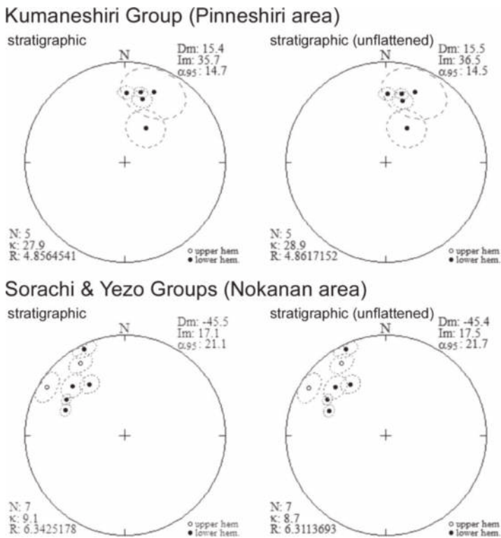
Figure 9. The primary magnetic directions of the Kumaneshiri, Sorachi and Yezo Groups before and after inclination shallowing correction in stratigraphic coordinates on equal-area projections. Solid (open) symbols are on the lower (upper) hemisphere of the equal-area projections. Dotted ovals are 95% confidence limits of site-means.
