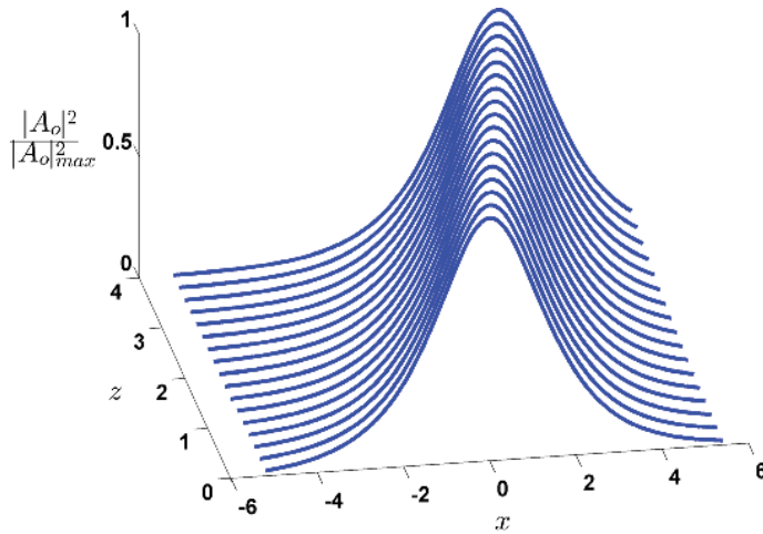
Figure 3. The self-trapped ordinary beam normalized intensity for the maximum amplitude |A_o|_{\max} = 10^5 \text{V/m} and \theta_o = \pi/6 .
