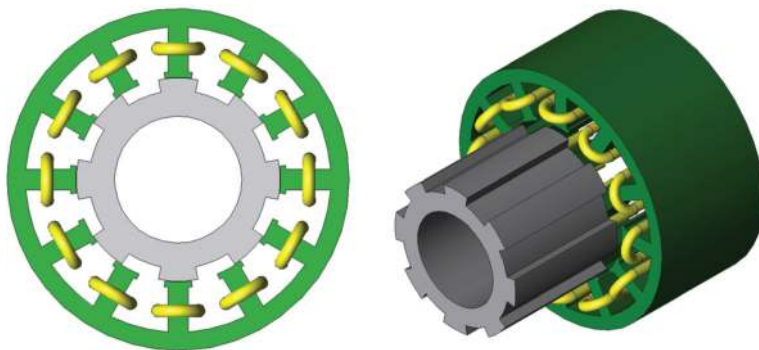
Figure 6. Three-phase 12/8-pole single-stator switched reluctance motor.
