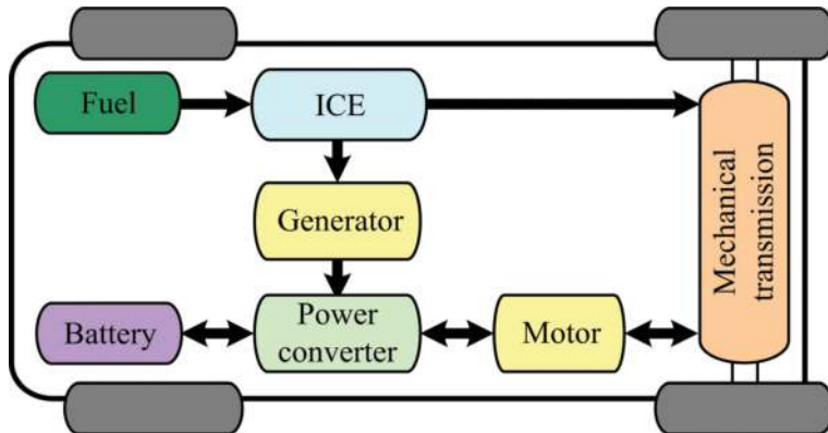
Figure 2. Parallel hybrid electric vehicle system.
