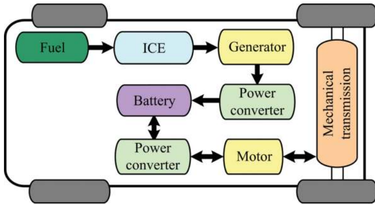
Figure 1. Series hybrid electric vehicle system.
