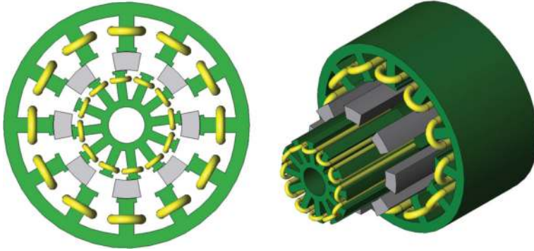
Figure 20. Three-phase 12/8-pole mechanical-offset double-stator switched reluctance motor.
