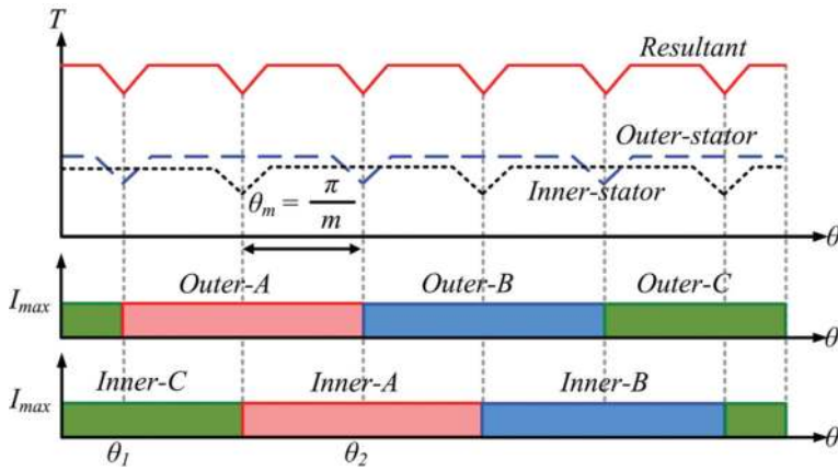
Figure 19. Operating principle for mechanical-offset double-stator switched reluctance motor.
