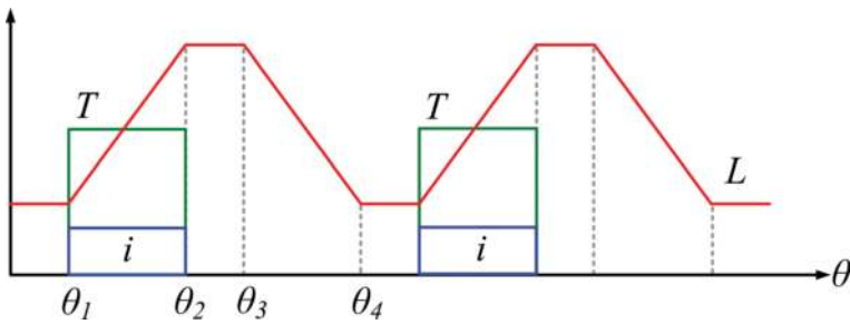
Figure 4. Theoretical operating waveform.
