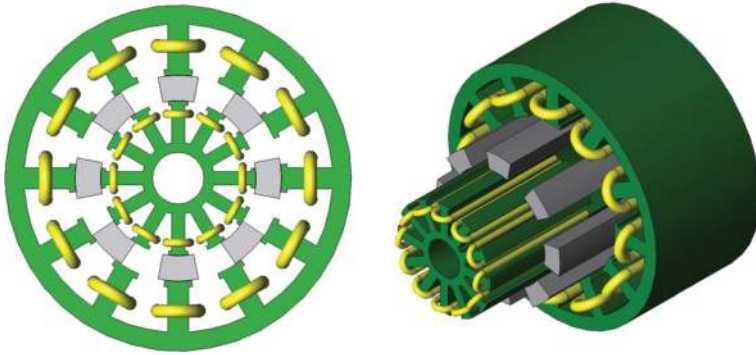
Figure 7. Three-phase 12/8-pole double-stator switched reluctance motor.
