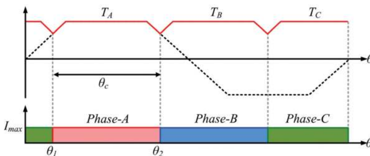
Figure 17. Operating principle for switched reluctance motor.
