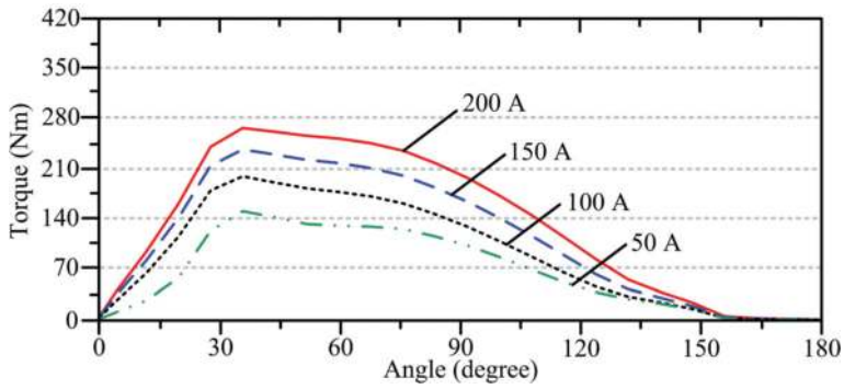
Figure 13. Torque capabilities of the switched reluctance motor.
