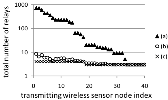
Fig. 11. Total number of relay wireless sensor nodes in 1-sink wireless sensor network. (a) q_i = -0.2 . (b) q_i = -0.6 . (c) distance level.
