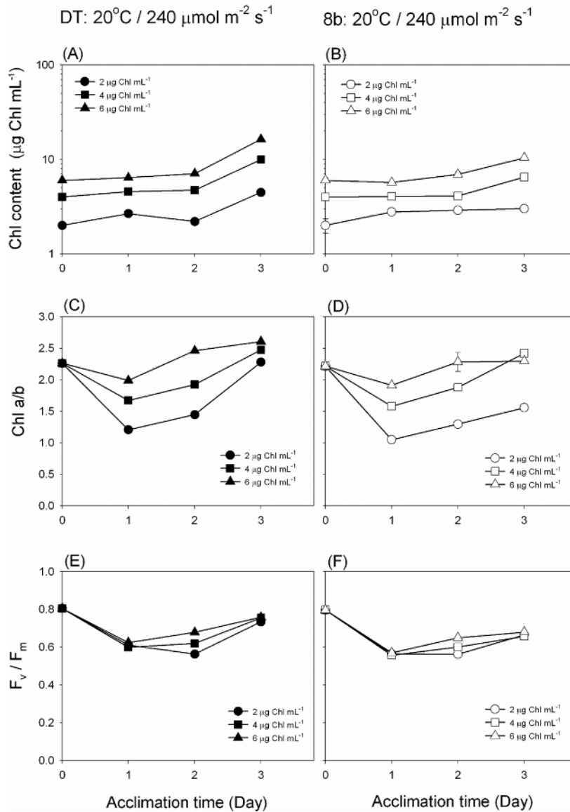
Figure 3. Effect of initial cultivation concentration on photosynthesis under 20°C and 240 μmol photon m -2 s -1 irradiance. The total Chl content (A, B), the Chl a/b ratio (C, D), and the F v /F m ratio (E, F) of Chlorella DT and 8b were measured in cultures with initial concentrations of 2, 4, and 6 μg Chl mL -1 at 20°C with irradiation of 240 μmol photons m -2 s -1 . Each point represents the average of two measurements from duplicate cultures (where not visible, error bars are smaller than the symbol).
