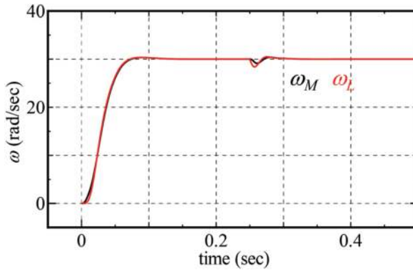
Figure 12. Simulation results when using the proposed method.
