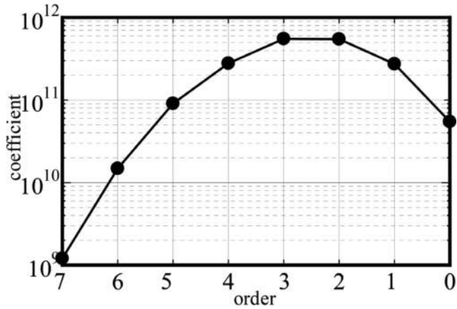
Figure 10. Designed coefficient diagram.
