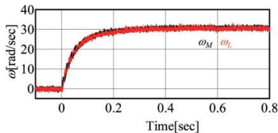
Figure 20. Experimental results obtained using conventional PI controller.
