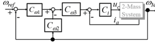
Figure 17. Simplified proposed control system.
