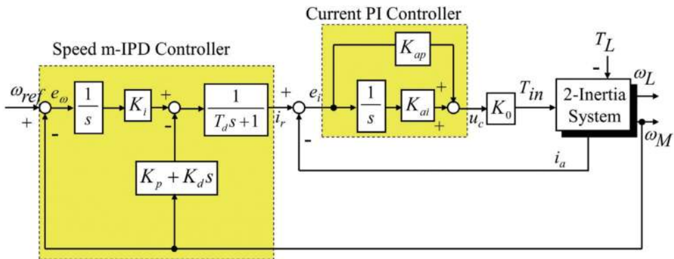
Figure 6. Proposed control system (continuous controller model).
