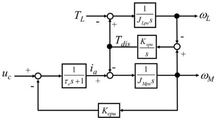
Figure 2. Block diagram of normalized two-mass resonance model.
