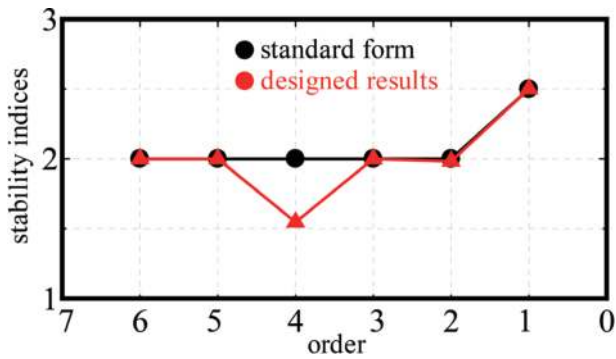
Figure 11. Designed and standard form stability indices.
