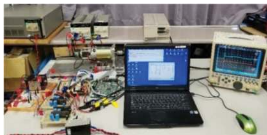
Figure 3. Overview of the experimental system.
