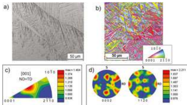
Figure 4. Microstructure of the FZ. (a) OM image of the microstructure, (b) orientation map in the cross section, (c) inverse pole figure, and (d) (0\ 0\ 0\ 1) and (1\ 1\ -2\ 0) pole figures in the cross section plane.
