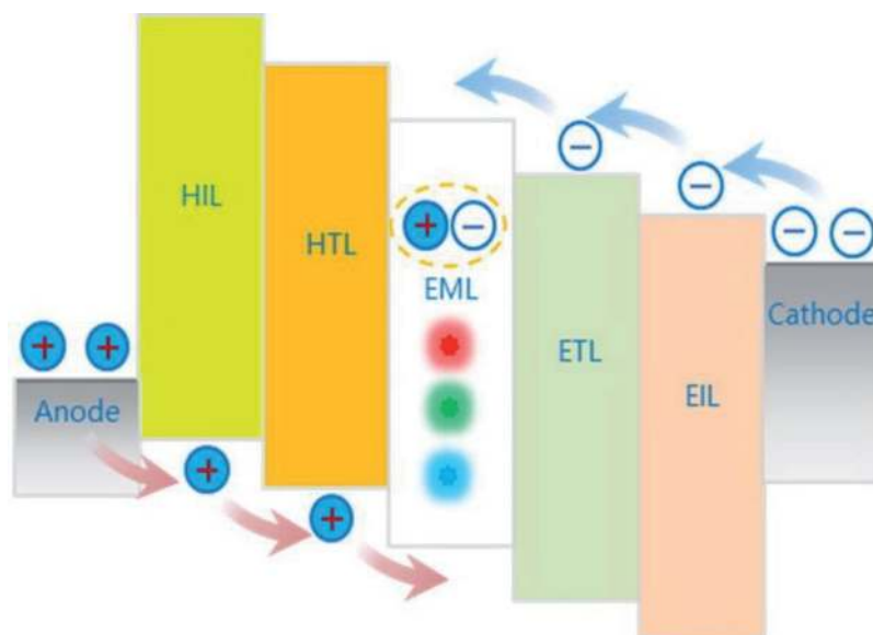
Figure 1. Structure of an OLED device.
