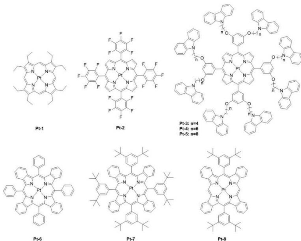
Figure 2. Chemical structures of platinum(II) porphyrin complexes Pt-1–8 .
