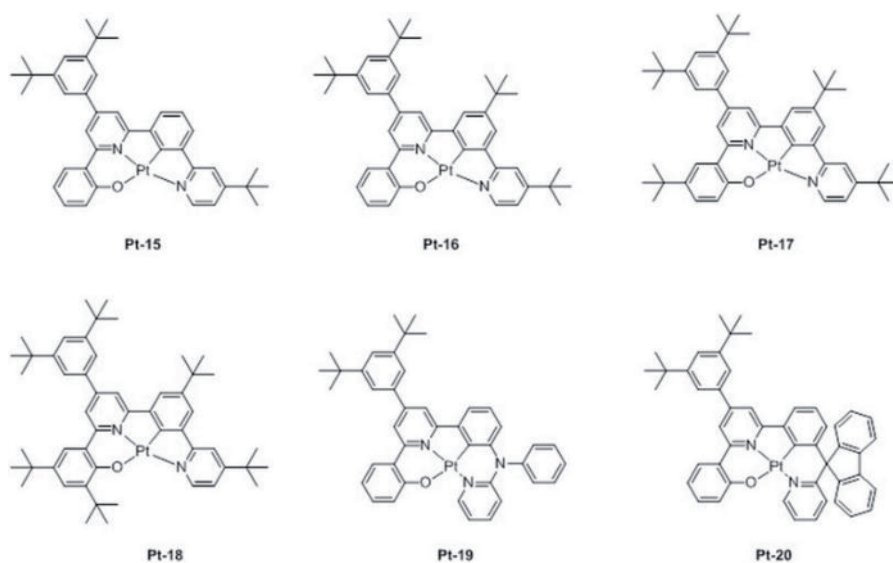
Figure 6. Chemical structures of platinum(II) complexes Pt-15–20 .
