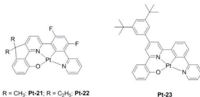
Figure 7. Chemical structures of platinum(II) complexes Pt-21–Pt-23 .
