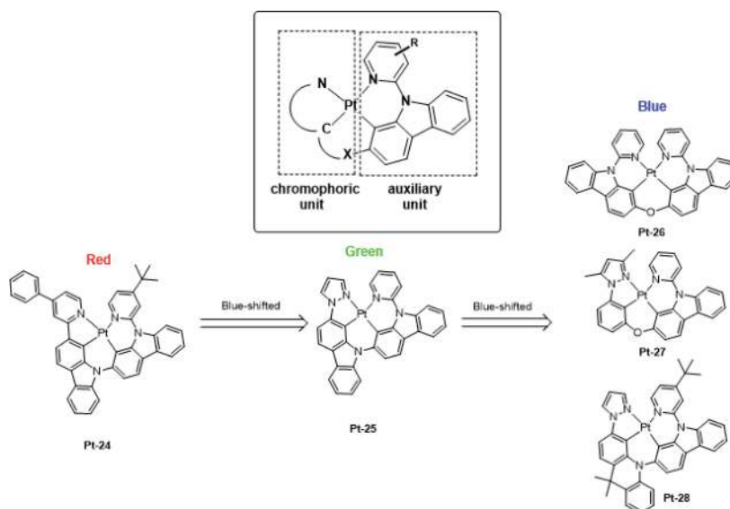
Figure 8. Molecular design strategies for color tuning.
