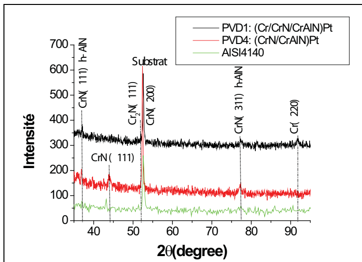
Fig. 2. Diffraction spectra of x-rays obtained with the multi-layer PVD1, PVD4 and steel 42CrMo4.
