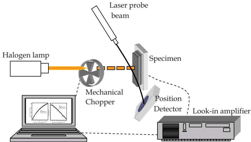
Fig. 9. Experimental set-up
