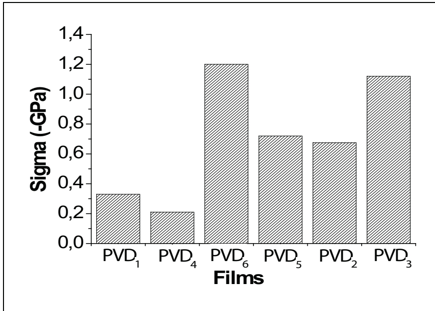
Fig. 11. Multi-layers Residual stresses
