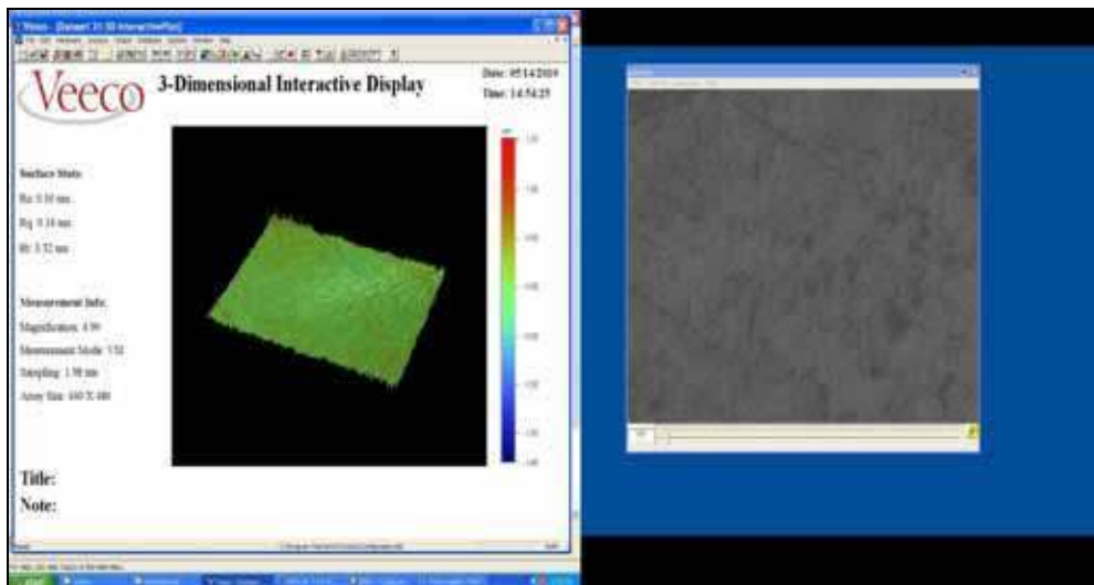
Fig. 1. Topography of coating PVD 1 obtained by the optical profilometer.
