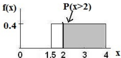
Figure 5.4: Uniform Distribution between 1.5 and 4 with shaded area between 2 and 4 representing the probability that the repair time x is greater than 2
