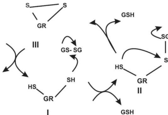
Figure 1. Schematic representation of the GSSG reduction cycle by GR.
