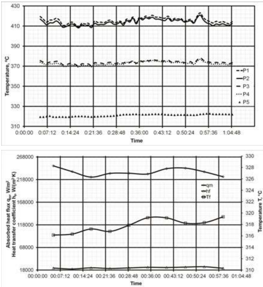
Figure 13. Measured temperature histories at five points for heat flux tube located at the level of 15.4 m (a) and estimated parameters: absorbed heat flux q_m , Heat transfer coefficient h_t and fluid temperature T_f (b).
