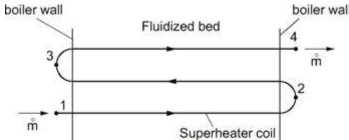
Figure 28. Three pass single superheater coil.
