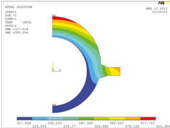
Figure 8. Temperature distribution in the flux-tube cross section for: q_m = 150000 \text{ W/m}^2 , T_i = 317^\circ\text{C} and h_f = 27000 \text{ W/(m}^2 \text{K)} .
