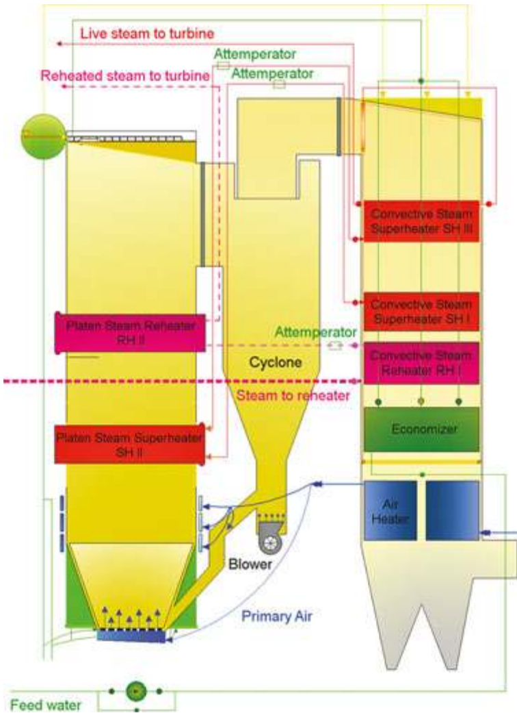
Figure 17. The arrangement of heating surfaces in circulating fluidized bed boiler with a steam capacity of 425 \cdot 10^3 kg/h.
