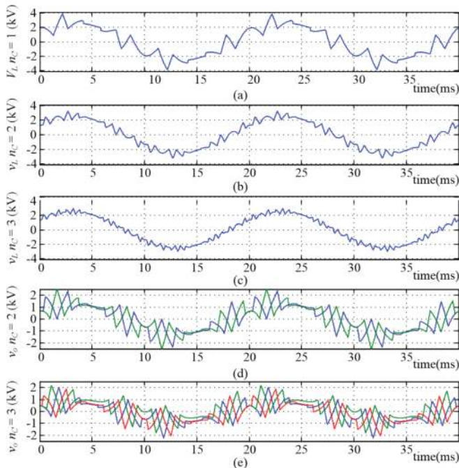
Figure 5. Voltage features for n_C = 1 , n_C = 2 , and n_C = 3 , C_o = 17\mu\text{F} ; (a) load voltage for n_C = 1 (THD = 28.2%), (b) load voltage for n_C = 2 (THD = 14.2%), (c) load voltage for n_C = 3 (THD = 9.6%), (d) capacitor voltage for n_C = 2 , and (e) capacitor voltages for n_C = 3 .
