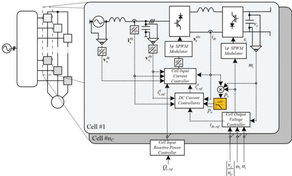
Figure 10. A control scheme for an AC drive based on CHB-CSL.
