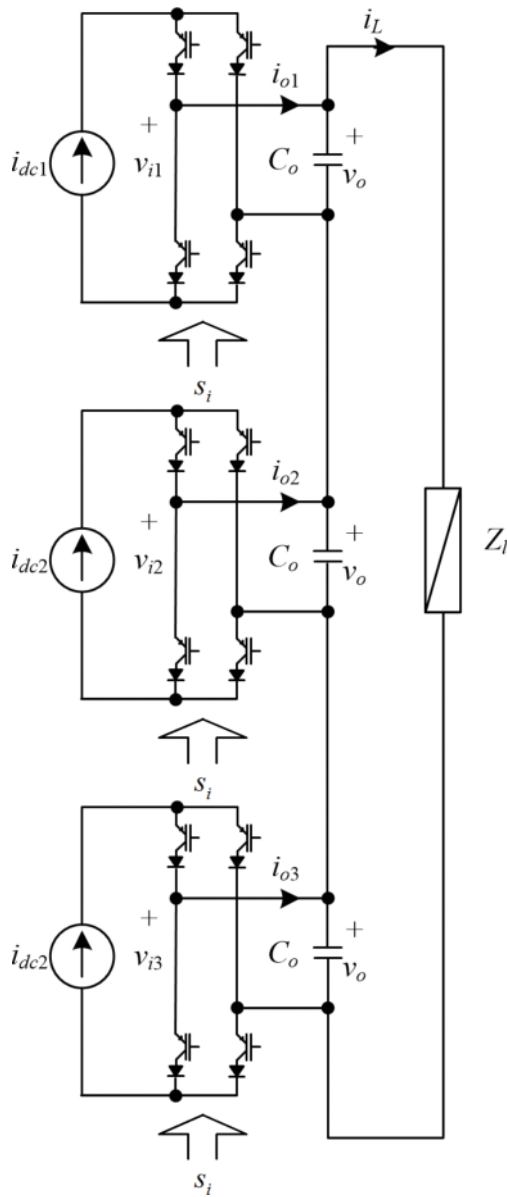
Figure 4. Three-phase applications of CSC-CHB ( n_c = 3 ).
