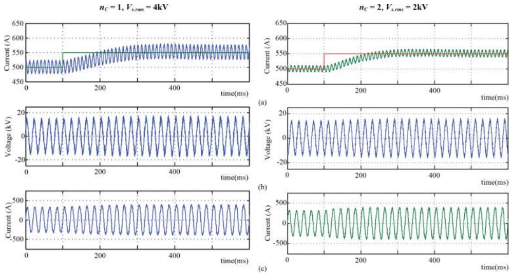
Figure 15. Key waveform for 10% DC current step (a) DC current, (b) load voltage, and (c) cell input current.
