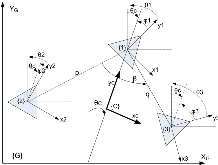
Fig. 8. Reference frame definition placing the cluster center at the triangle centroid
