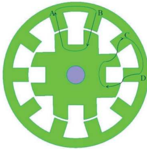
Figure 13. A short-flux path MRS configuration.
