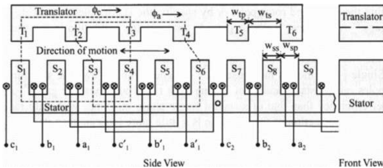
Figure 11. LSRM structure.
