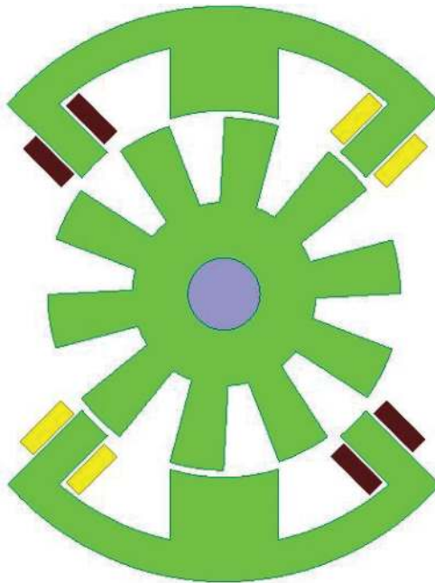
Figure 14. A common pole E-core SRM configuration.
