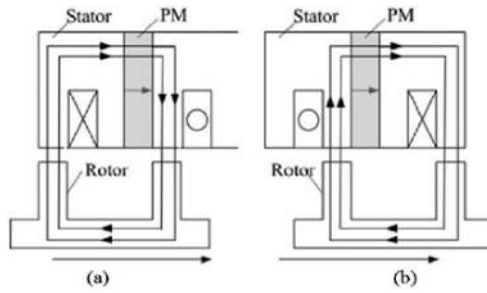
Figure 19. Operational principle of a flux-switching motor.
