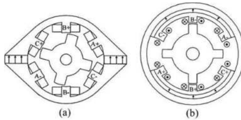
Figure 17. Two unidirectional flux PM-assisted motors.
