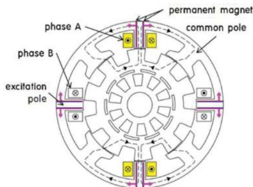
Figure 24. The flux path in a PM-assisted SRM.
