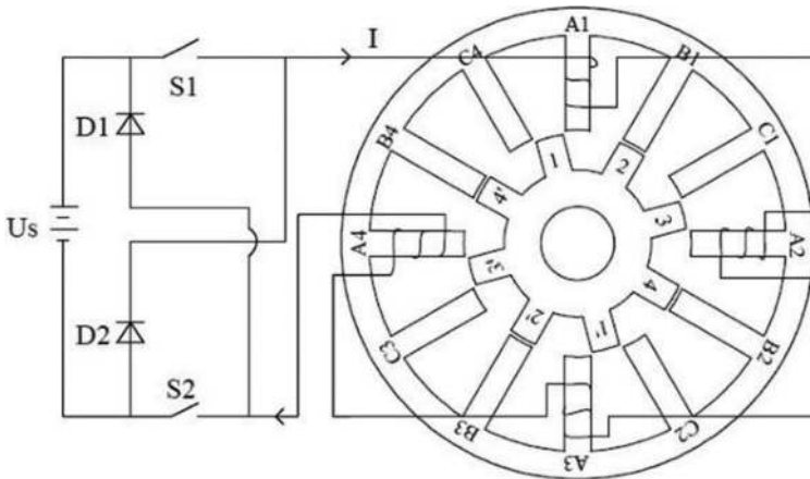
Figure 9. A 12:8 pole three-phase SRM generator configuration.
