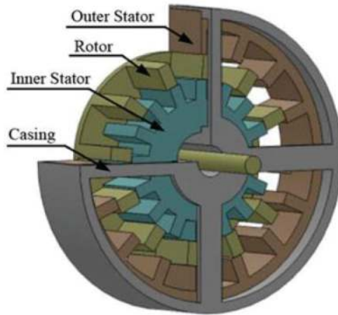
Figure 28. Primary 3-D model of designed DSSCR-SRM.
