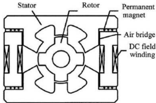
Figure 23. A hybrid-excited DSPM motor.
