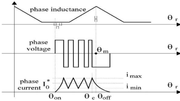
Figure 7. Current and voltage control in a phase below the base speed using PWM converter.
