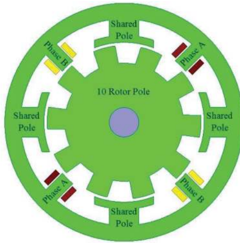
Figure 16. A common pole E-core SRM configuration.
