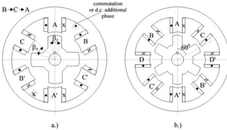
Figure 3. 6:4 three-phase and 8:6 four-phase configurations.
