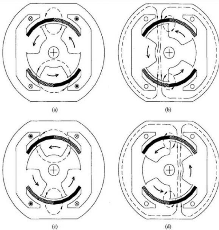
Figure 22. The functioning of flux reversal motors.
