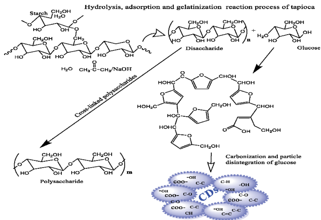
Figure 2. Mechanism for synthesis of carbon dots [2].
